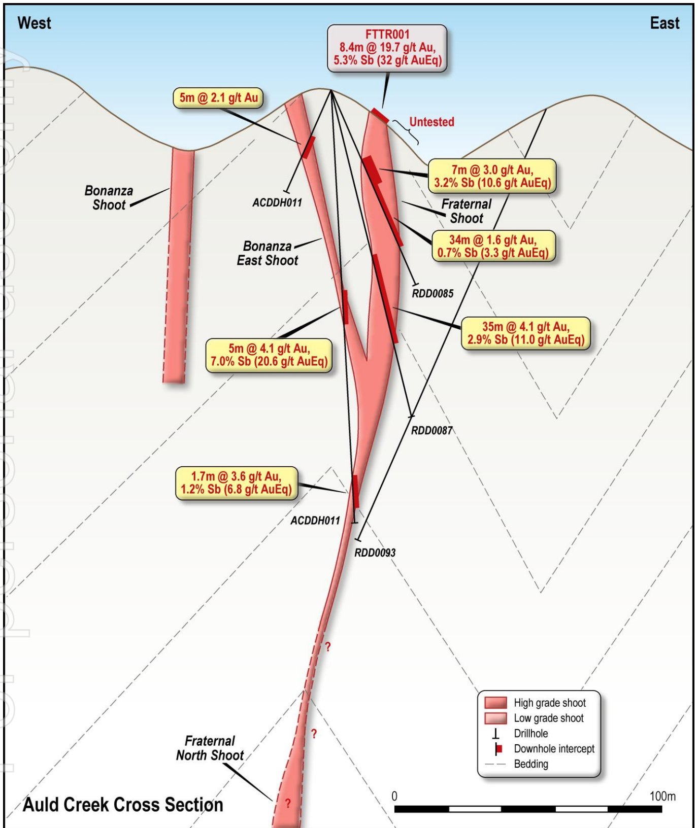
Figure 3. Auld Creek schematic cross section showing the potential Bonanza and Fraternal North Shoots.
