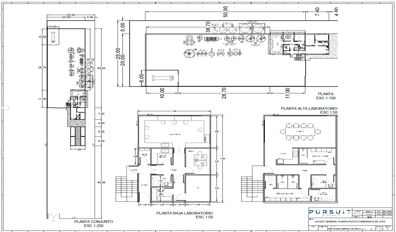
Figure 5 – Pursuit Lithium Carbonate 250tpa Plant Design Layout.
