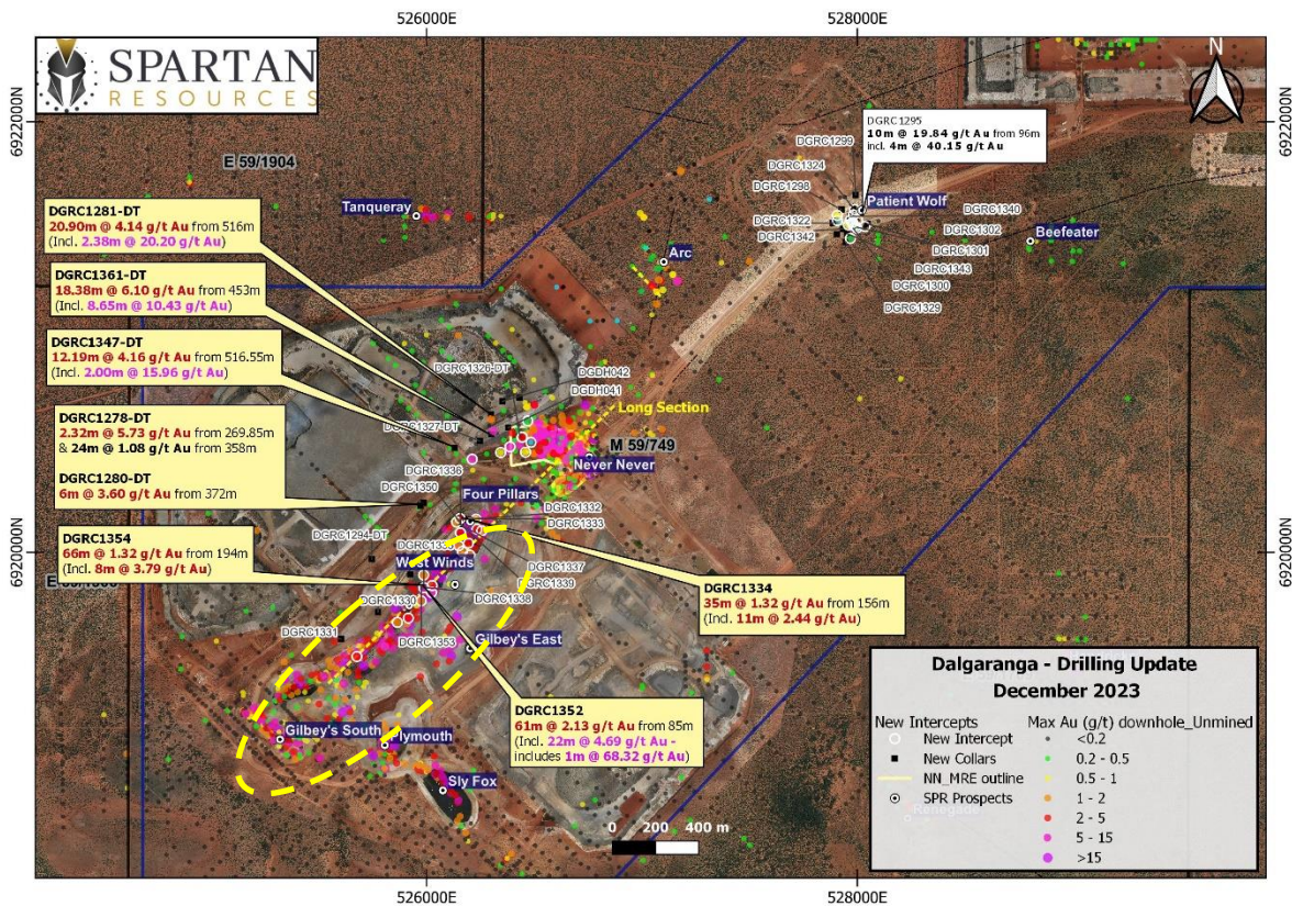
Figure 2: Plan view of the Dalgarganga Mine Complex with recent highlight drill assay results and drill collars coloured by grade across the Never Never gold deposit, Four Pillars and West Winds gold prospects (higher-grade sections of the larger Gilbey's open pit "yellow dash outline") and the Patient Wolf gold target to the north-east. Note the Granted Mining Lease boundary in blue.
