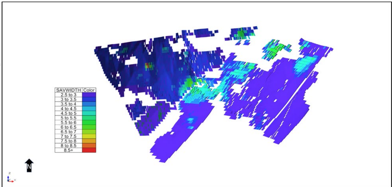
Figure 4-2 | Underground stoping widths in metres
