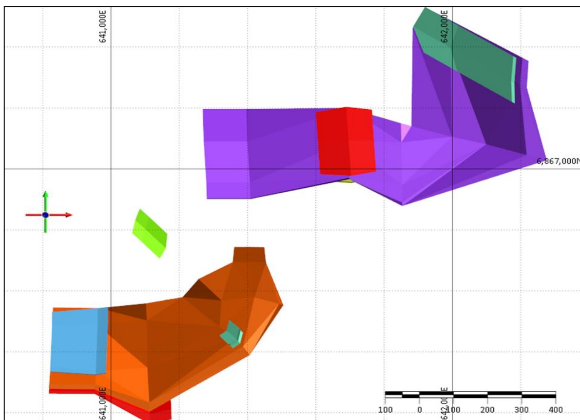
Figure 10; Plan view of Kinks wireframes – Wireframe colours by sub-domains with the main domain coloured orange which provides the largest contribution of mineralisation to the final MRE statement >0.5\% \text{ V}_2\text{O}_5 .
