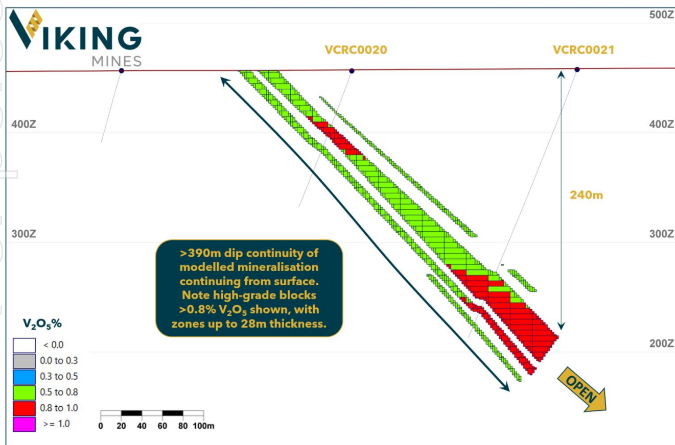
Figure 2; Cross-section through the Kinks Deposit looking to the West showing the distribution of high-grade zones within the broader mineralised package. Note mineralisation extends from surface to depth with over 390m dip continuity and thicknesses up to 28m.
