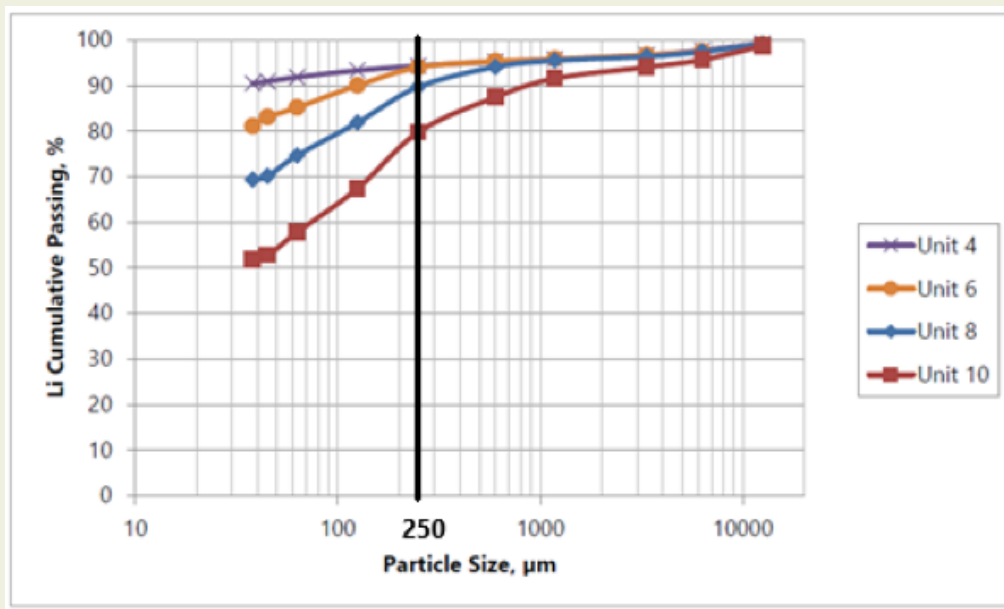
Figure 1 – Lithium Recovery to Leach Feed by particle size (Units 4, 6, 8 and 10)
