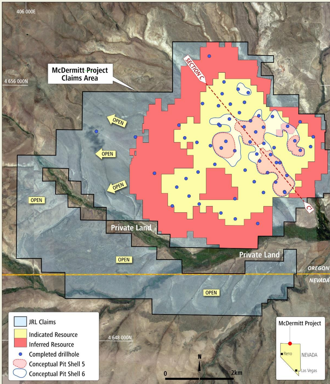
Figure 3 – Plan view of the McDermitt Lithium Project with 2023 Mineral Resource 1 (at 1523mRL), completed drilling, Section C-C' and schematic conceptual pit shells (Pit Shell 5: nominal 20 years; Pit Shell 6: nominal 43 years).
