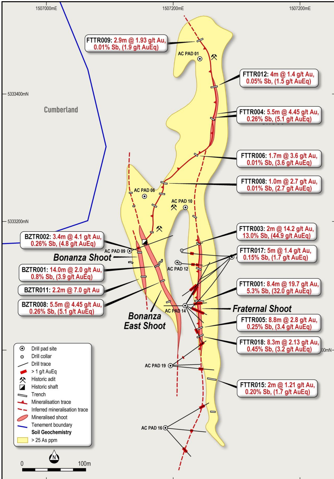
Figure 3. Auld Creek drillhole plan showing downhole intersections.
