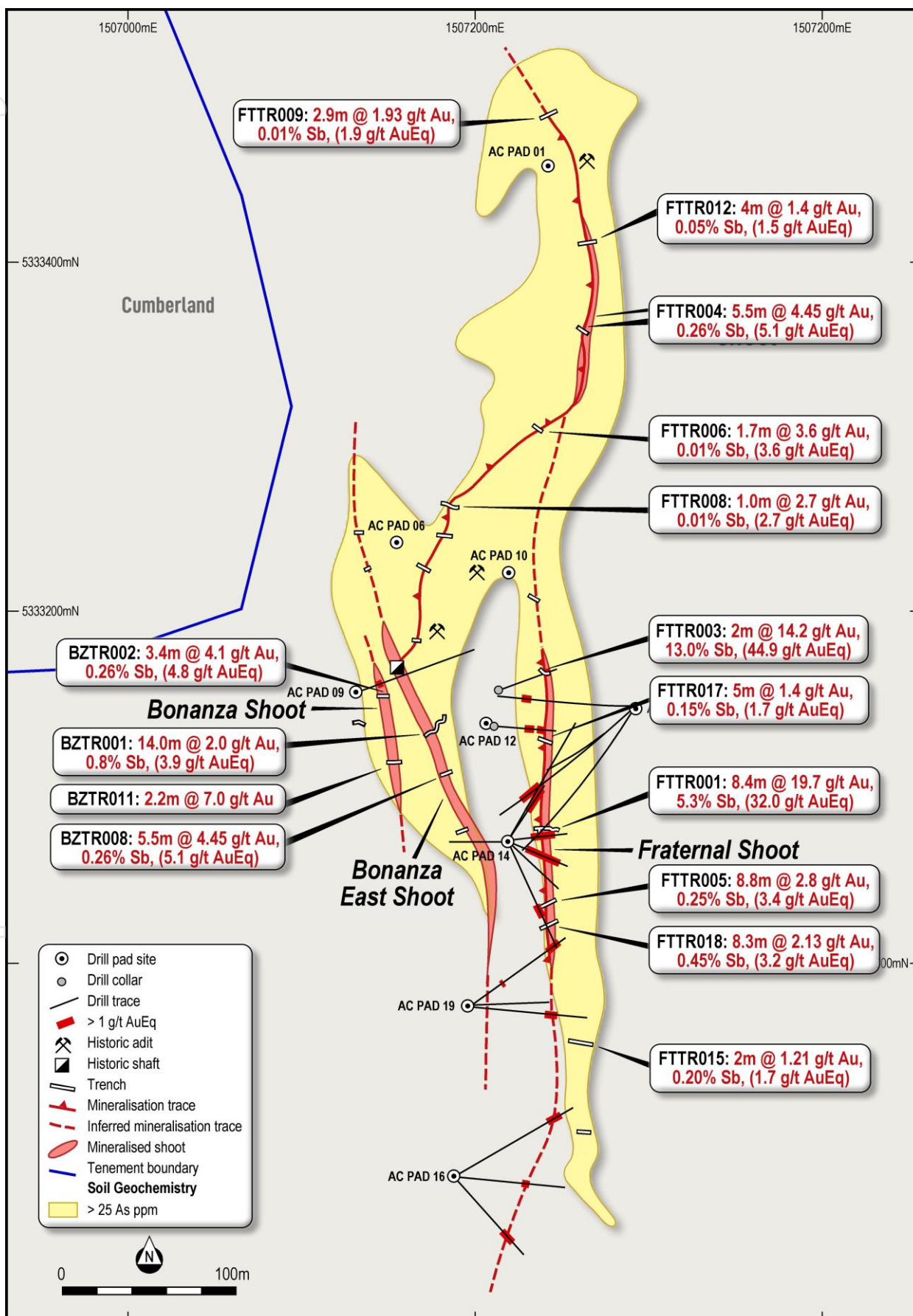
Figure 2. Auld Creek arsenic soil and trench plan.
