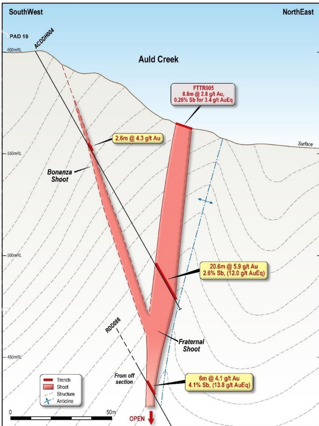
Figure 4. Auld Creek schematic cross section through ACDDH004 and RDD086.
