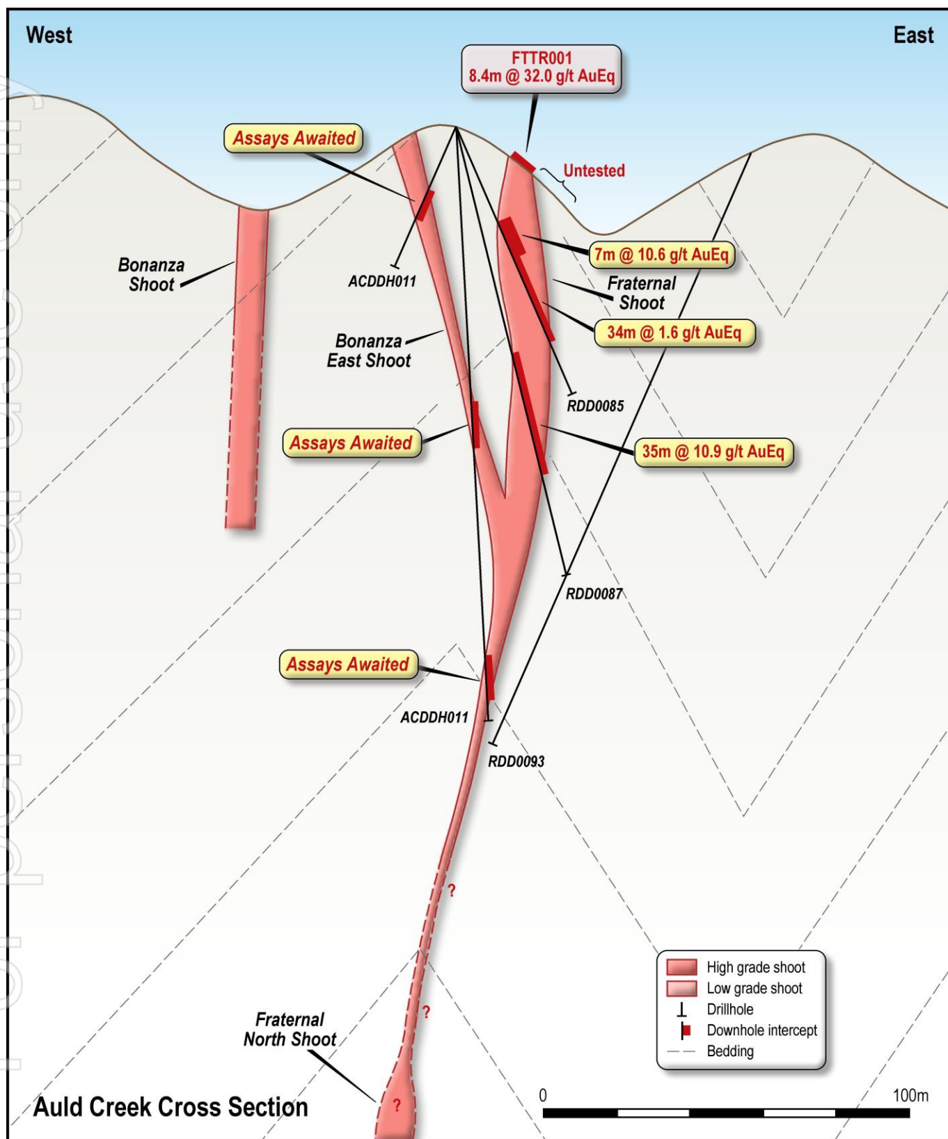
Figure 6. Extended Ald Creek schematic cross section showing the potential Bonanza and Fraternal North Shoots.
