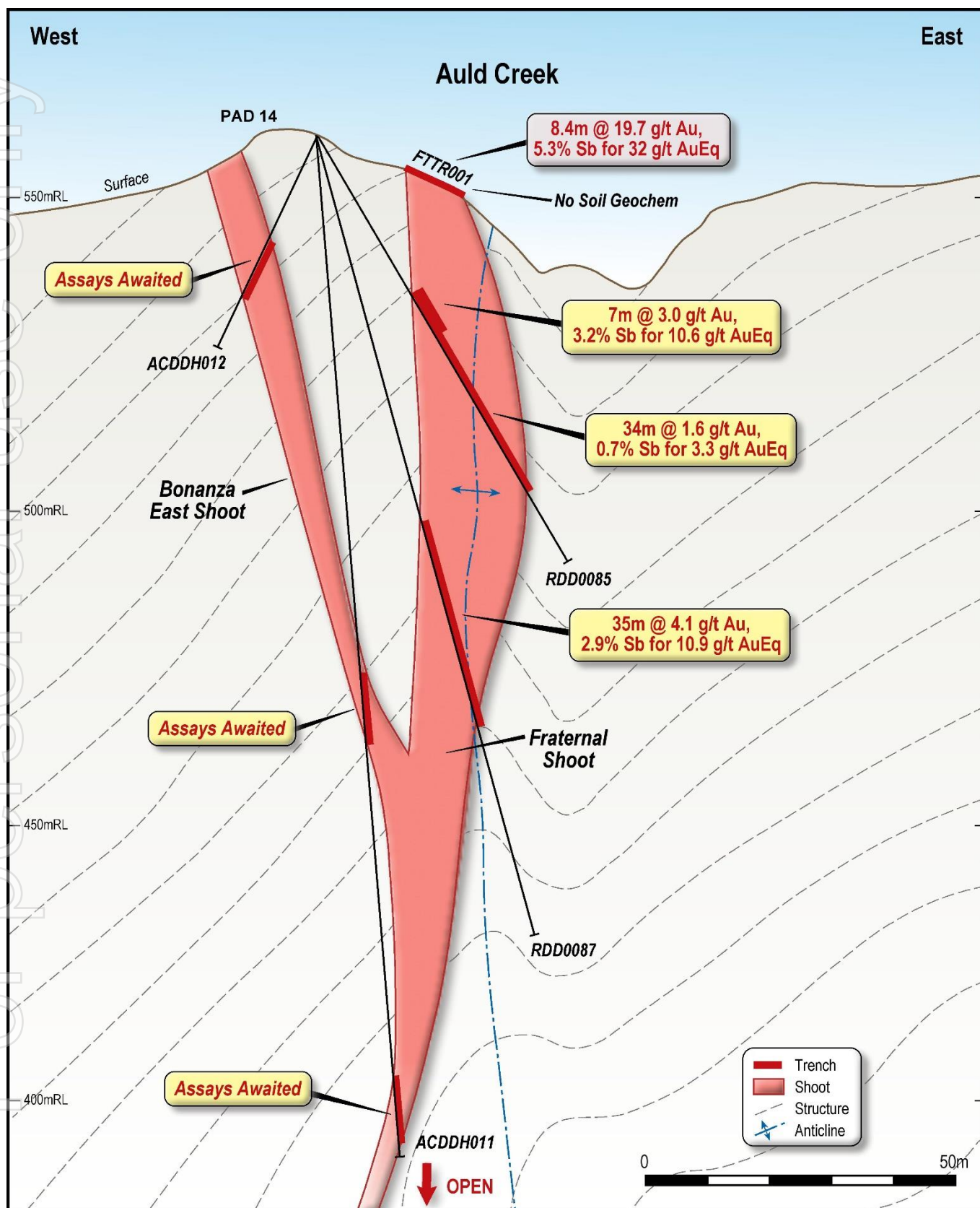
Figure 5. Auld Creek schematic cross section through RDD085, RDD087, ACDDH011 and ACDDH012.
