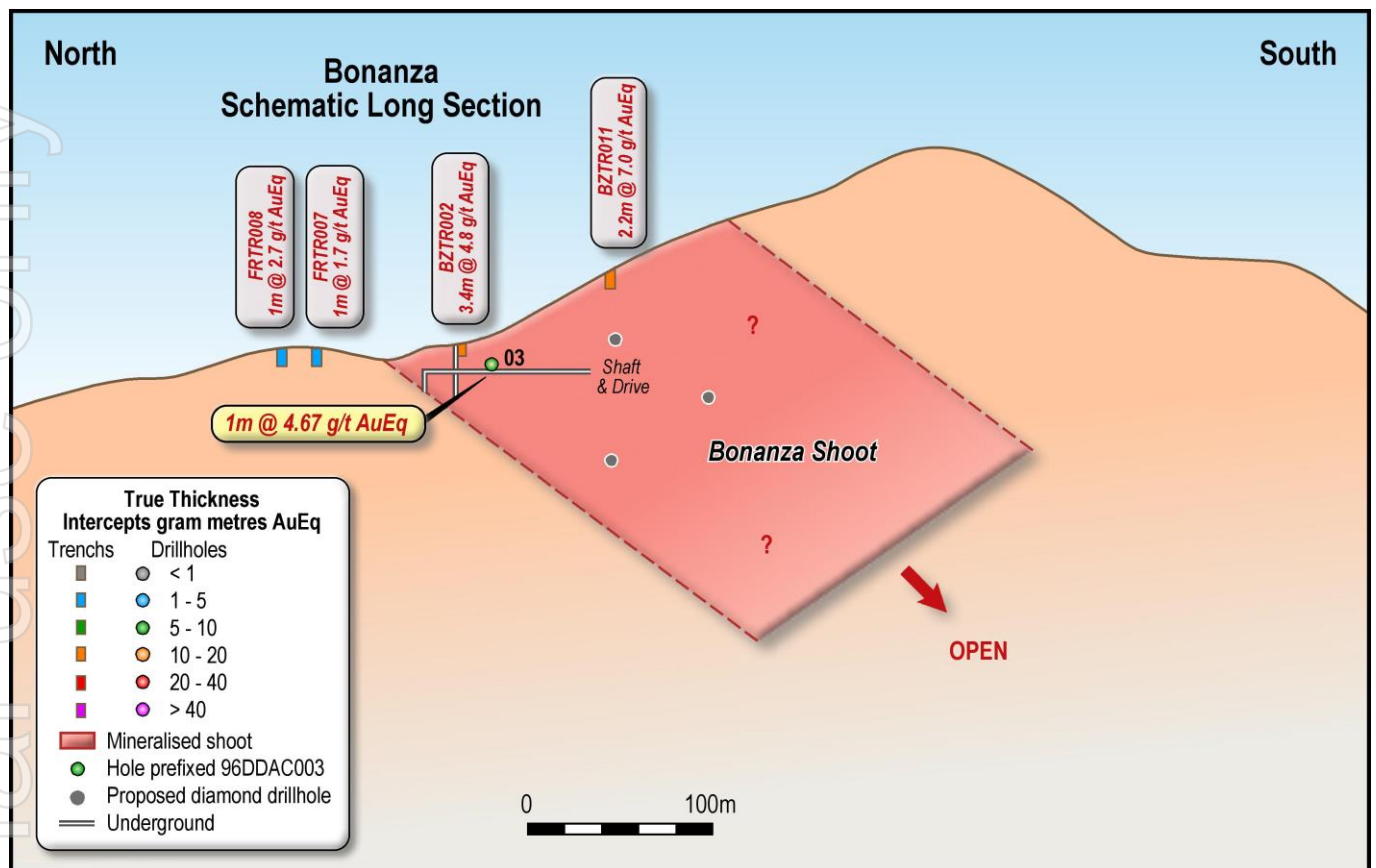
Figure 13. Bonanza Shoot schematic long section.
