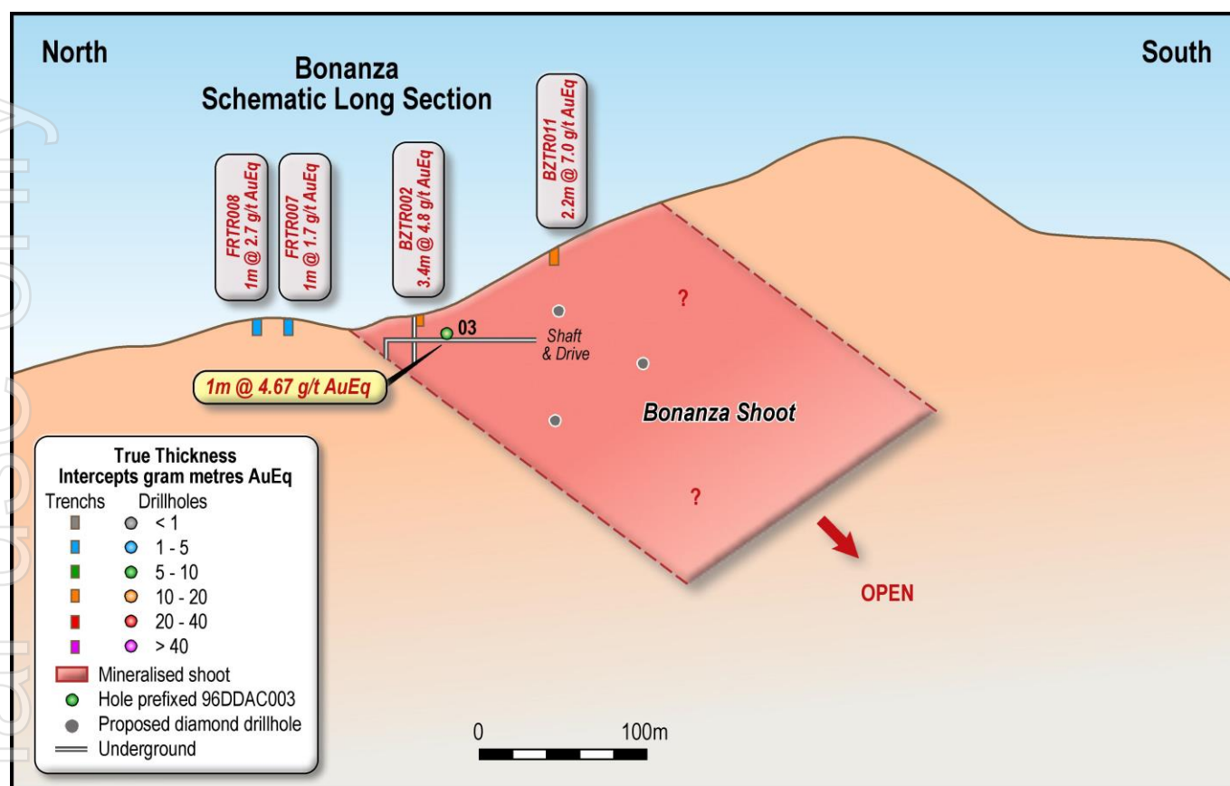
Figure 13. Bonanza Shoot schematic long section.
