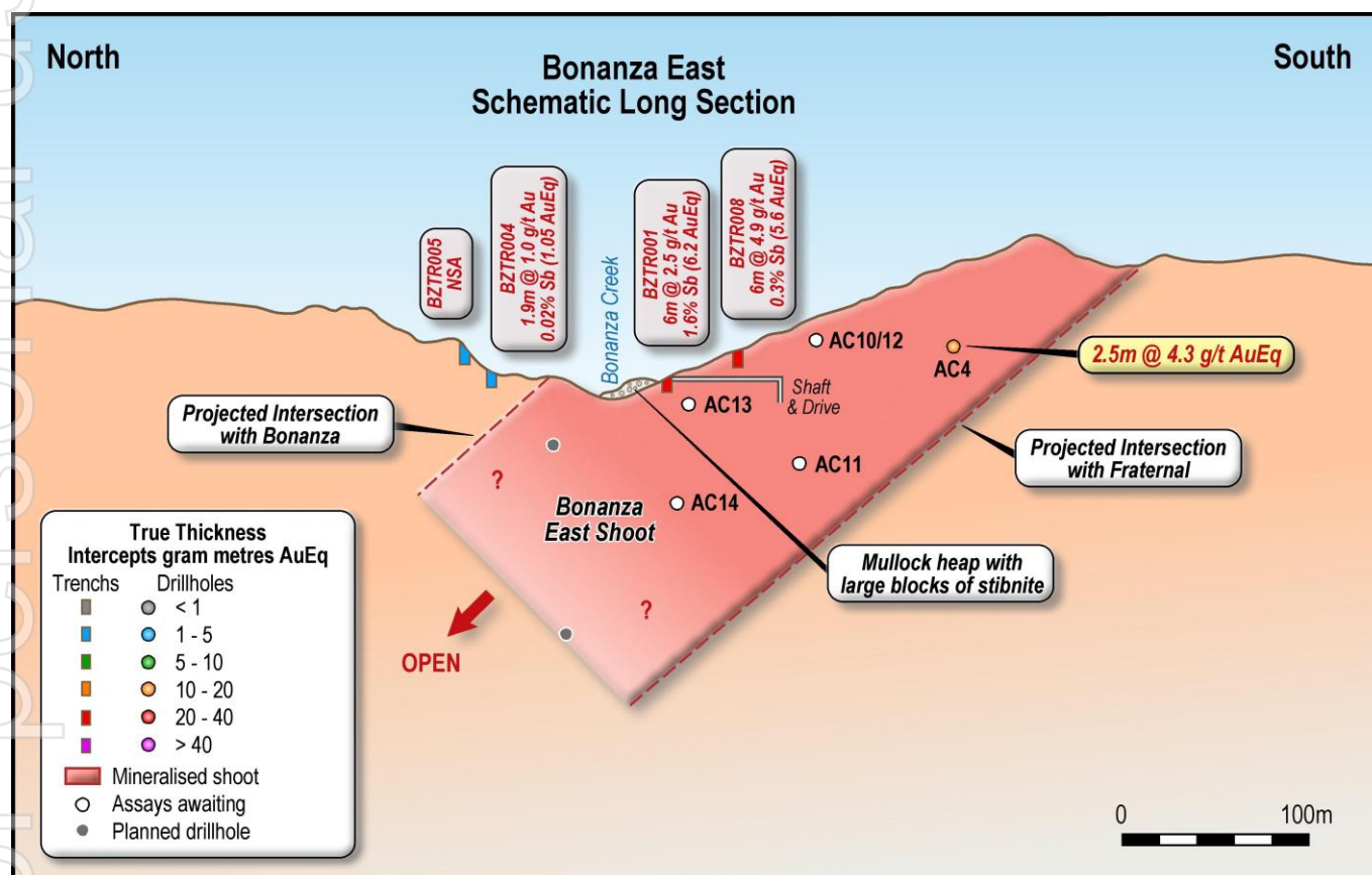
Figure 9. Bonanza East Shoot schematic long section.
