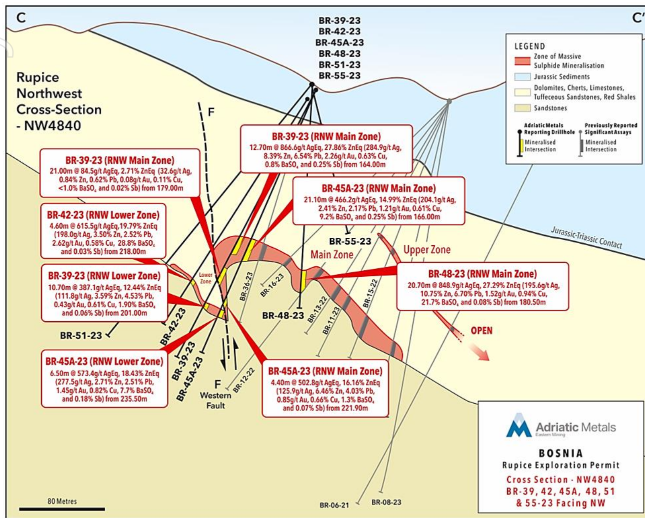
Figure 5: Cross-section (C-C') through BR-39-23, BR-42-23, BR-45A-23, BR-48-23, BR-51-23 and BR-55-23
