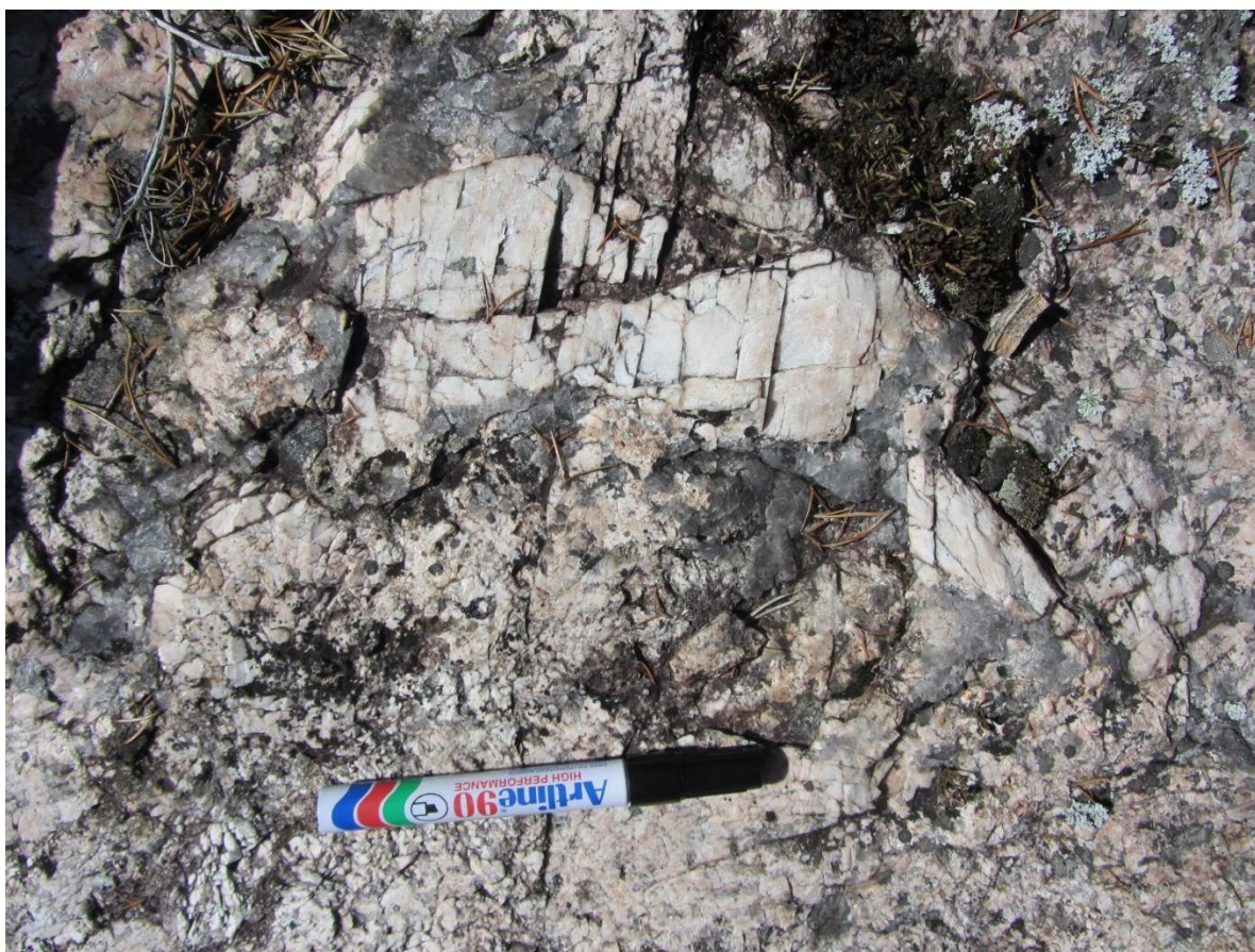
Figure 4 Megacrystic K-feldspar and quartz in the pegmatite
