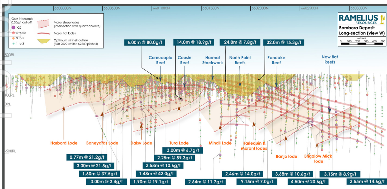
Figure 6: Roe - Bombora deposit cross-section June 2023 - drilling and lode interpretation
