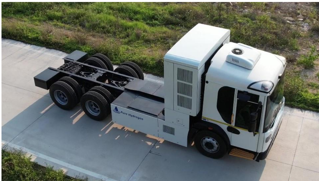
Image 1: An aerial image of Pure's first hydrogen fuel cell waste collection vehicle, which is now being fitted with refuse collection components by Bucher Municipal.
