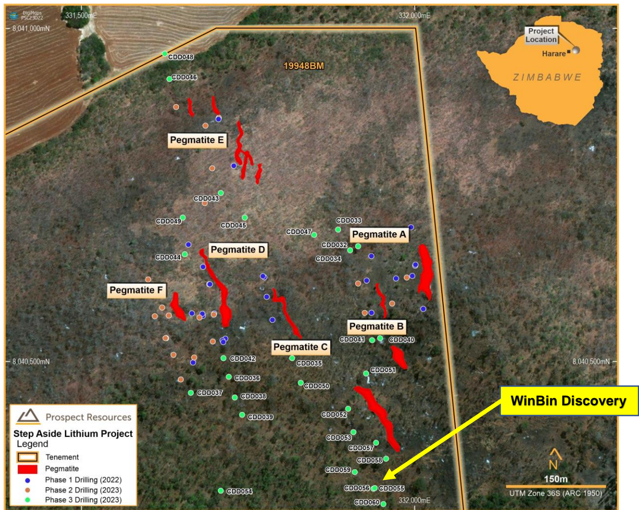
Figure 3: Plan view showing Phase 3 diamond drilling at Step Aside and WinBin Discovery
