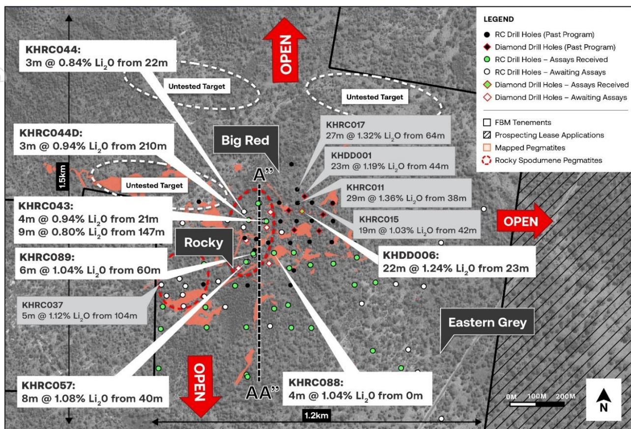
Figure 1: KHLP North – Big Red and Rocky Prospects In Plan View
