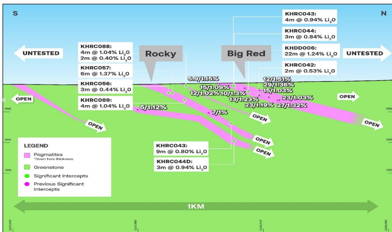
Figure 2: KHLP North – Long Section
