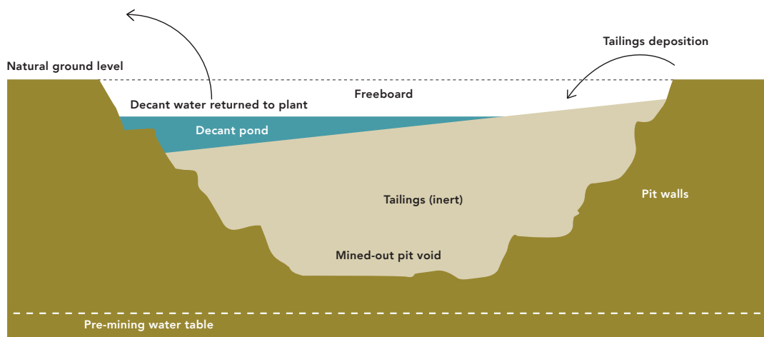
Figure 26: In-pit type TSF (Ghost Crab TSF is an example of this type of facility)
