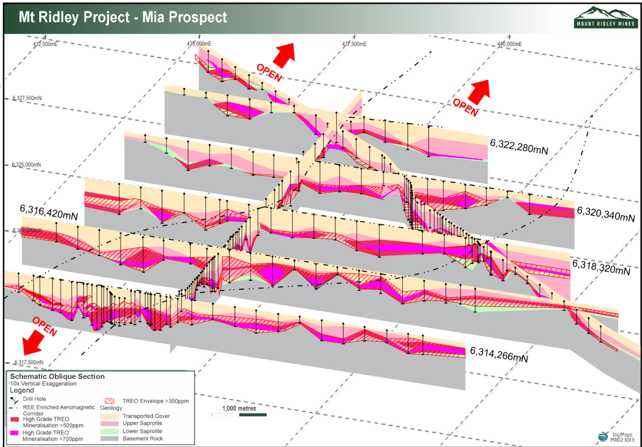
Figure 4: Mia Prospect aircore drilling. Stacked cross sections show drill holes and layered REE mineralisation. The grid lines are 2.5 km apart. The vertical scale is 10x the horizontal scale.
