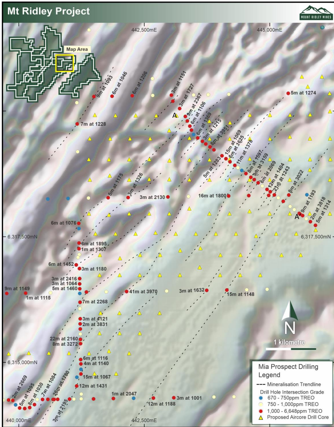
Figure 3: 100m-spaced drill holes demonstrate that highly enriched REE mineralisation is continuous between earlier drill holes which were spaced at 400m intervals. Mineralisation often occurs along linear, magnetic 'ridges' seen in aeromagnetic imagery. Red dots are significant intersections with an average grade >1000ppm TREO (using a 700ppm TREO lower cut). Proposed infill drill holes are shown as yellow triangles.
