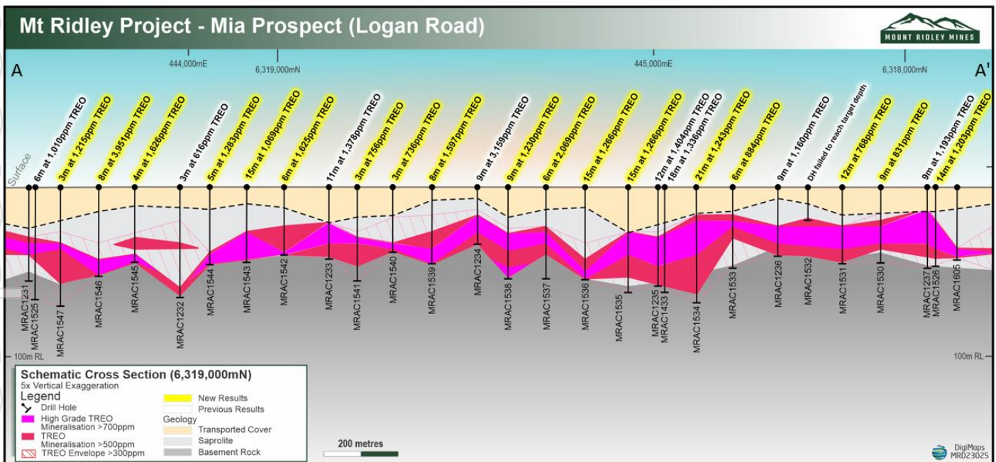
Figure 2: Cross section across the Mia Prospect, (refer to Figure 3 for location), which is 2.5km wide, showing thick zones of clay-hosted REE mineralisation. Drill holes are 100m apart. Infill holes are shown with yellow highlight. The vertical scale is 5x the horizontal scale.
