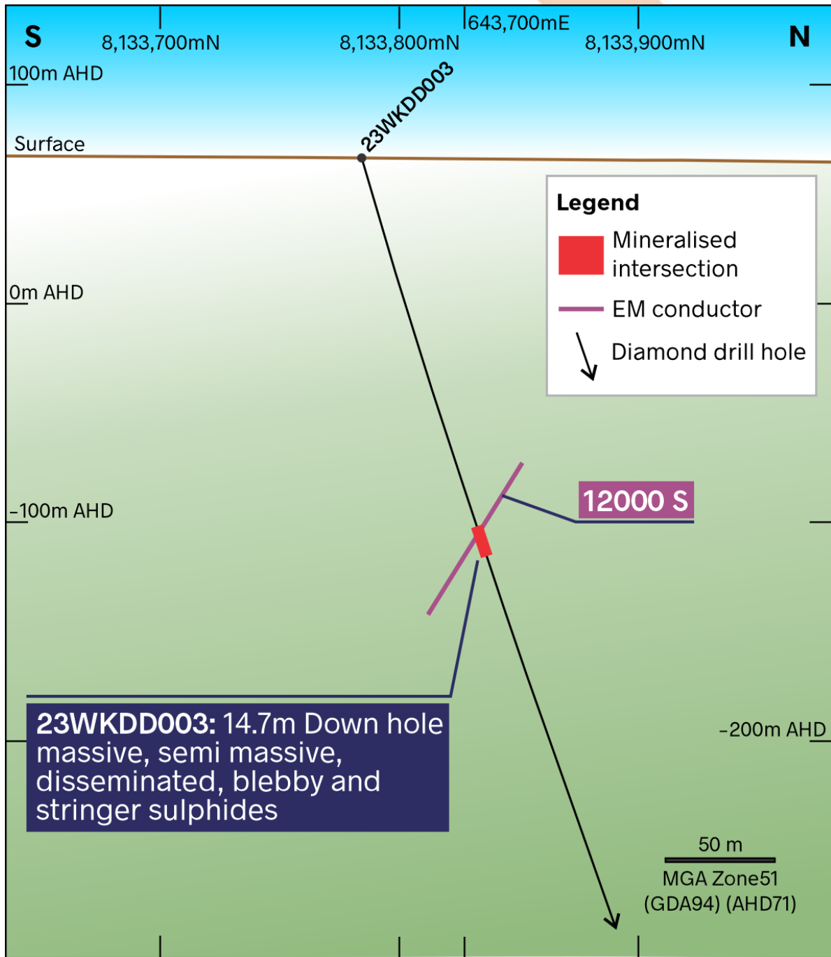
Figure 4: North-South Section showing the Dogleg EM Conductor, the diamond drillhole trace, and intersected sulphide mineralisation detailed in Table 1 (14.7m of visual sulphide mineralisation from 176.45 m downhole).
