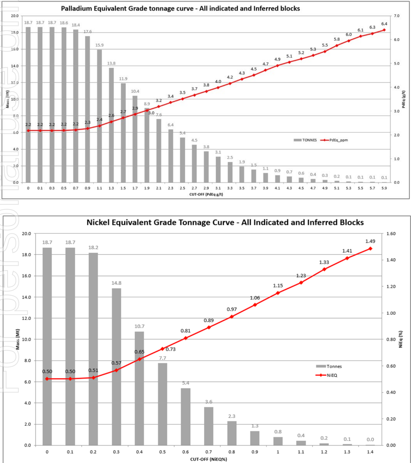
Figure 2 - Grade-tonnage curves for the Callisto Deposit (PdEq in upper chart and NiEq lower chart)
