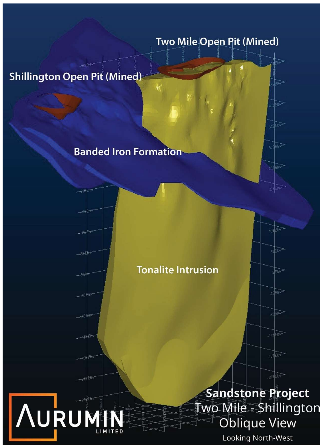
Figure 2. Oblique view toward the Northwest showing major geological units within the Shillington- Two Mile hill complex. The blue wireframe is the Banded Iron Formation unit and the yellow wireframe is the tonalite intrusion.
