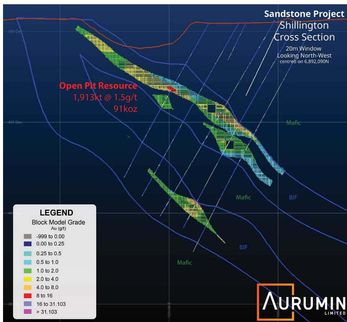
Figure 5. Shillington mineralisation interpretation indicative cross section, showing block model and drilling. Looking northwest, centred on 6,892,090N
