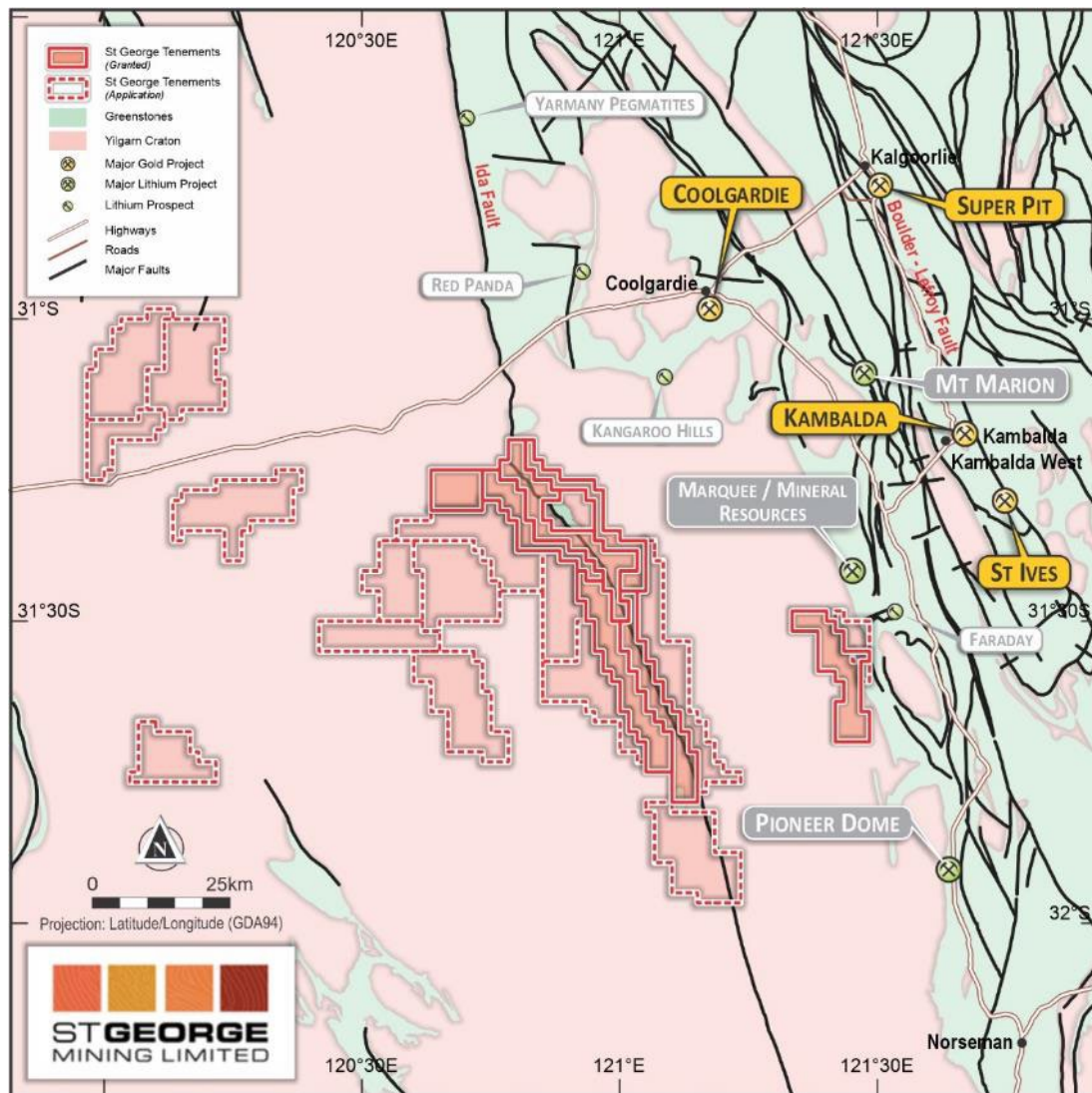
Figure 8 – map showing the regional location of the Woolgongie Project.
