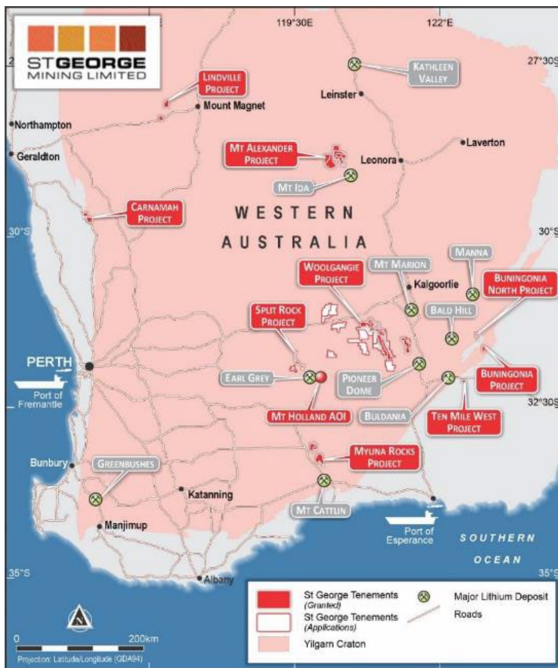
Figure 1- map of the south-east Yilgarn of Western Australia showing St George's multiple projects in the region as well as major lithium mines and deposits.
