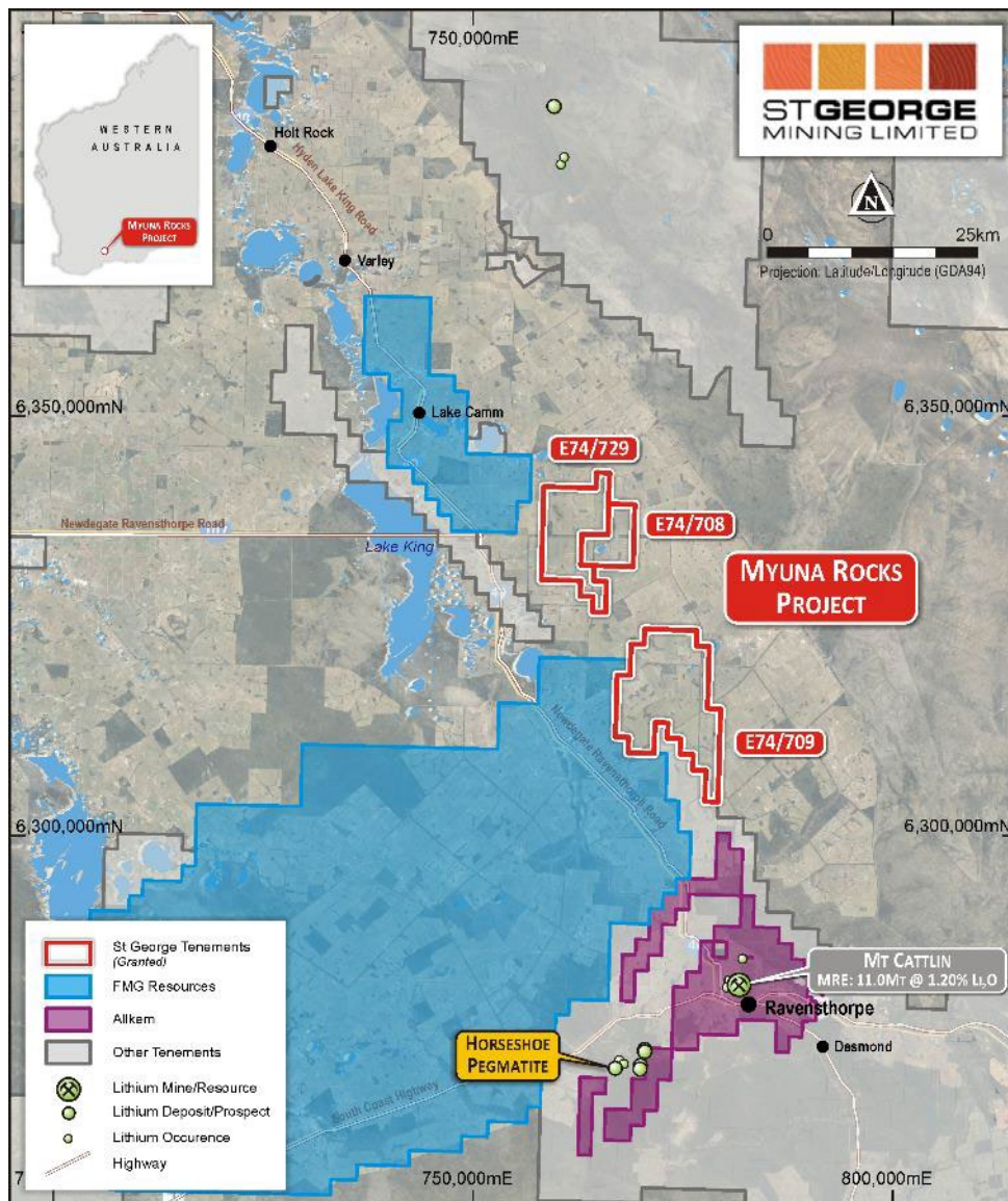
Figure 7 – map showing the location of the Myuna Rocks tenements, highlighting the nearby Mt Cattlin lithium mine and the large landholding of Fortescue Metals Group (ASX: FMG).
