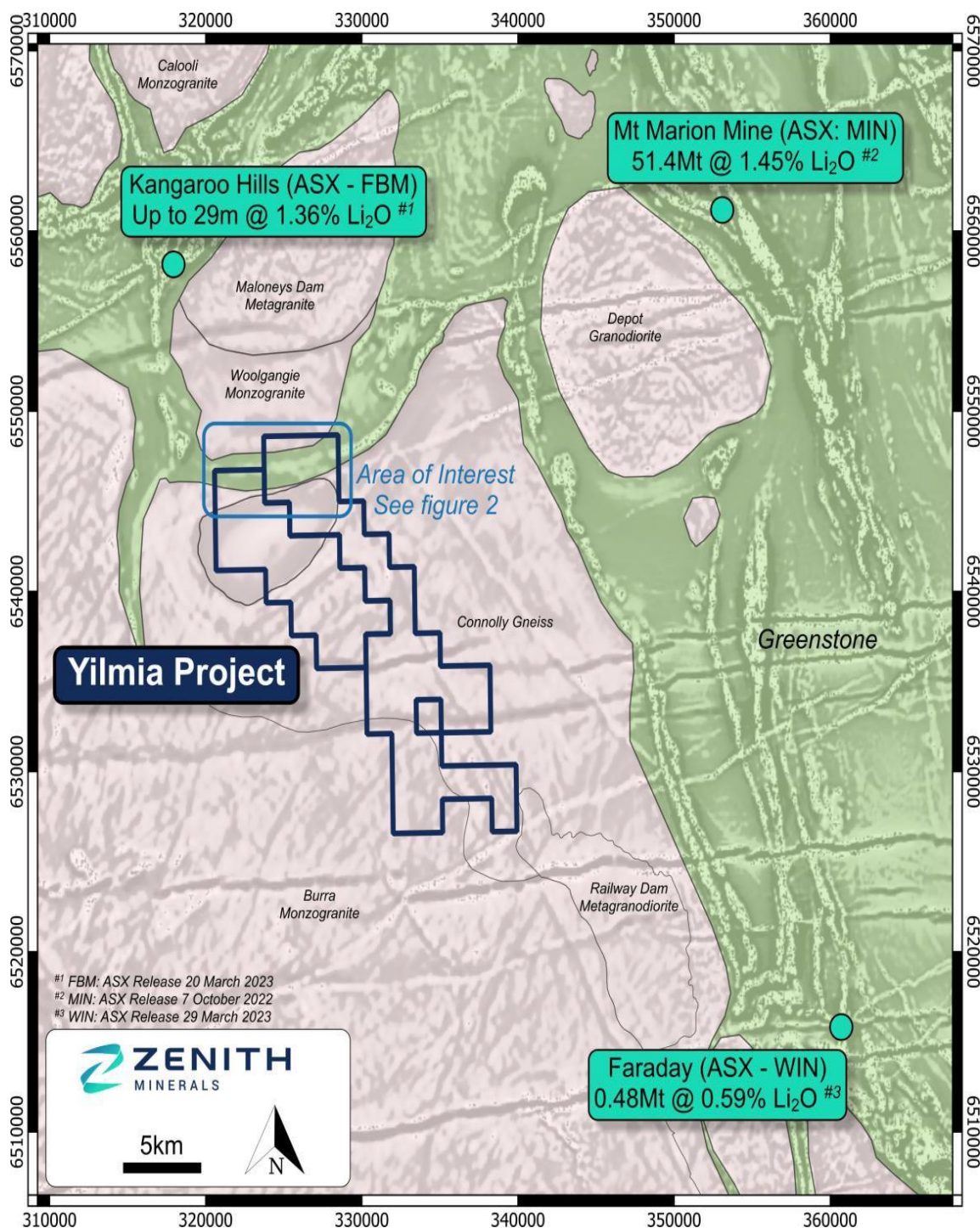
Figure 9: Yilmia Lithium Project - Location Map (Greenstone Outlines over Aeromagnetic Greyscale _ RTP Image)
