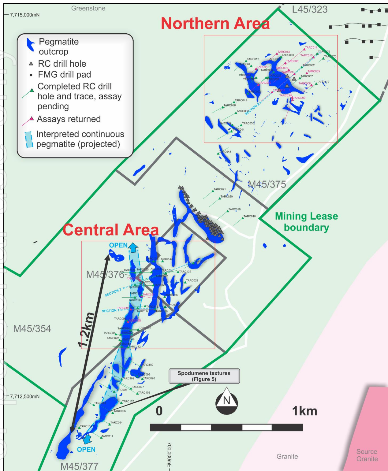
Figure 1 – Tabbatabba Project showing outcropping pegmatites in blue and the collar locations of the holes (green triangles) drilled to date. The central area and northern areas are highlighted in red. Note that the thick pegmatite intercepted in TARC089, TARC087 and TARC023 is highlighted in light blue and appears continuous and open over 1.2km and averages 40m width in all intercepts to date, with a peak width of 132m.
