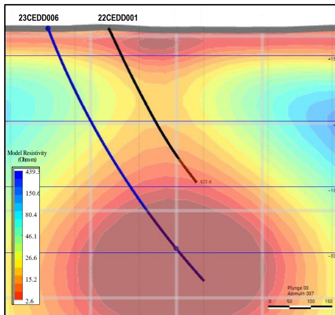
Figure 2: Central exploration target AMT anomaly showing drill hole traces of hole 6 and hole 1.
