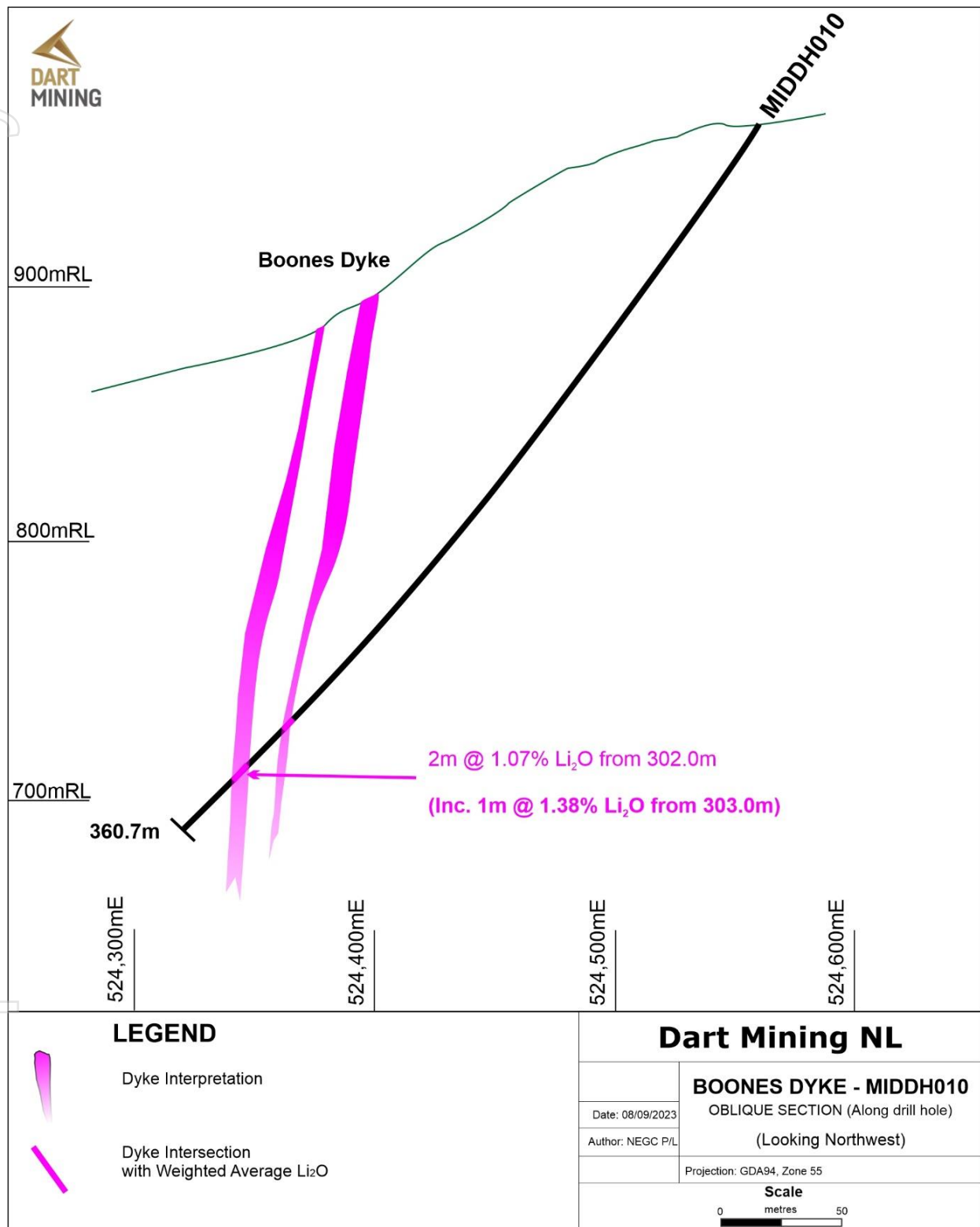
Figure 2 - Cross-section interpretation of drill hole MIDDH010 with assay highlights from Boones Dyke.
