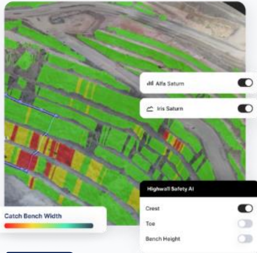
AI Enabled Highwall Safety Analysis
