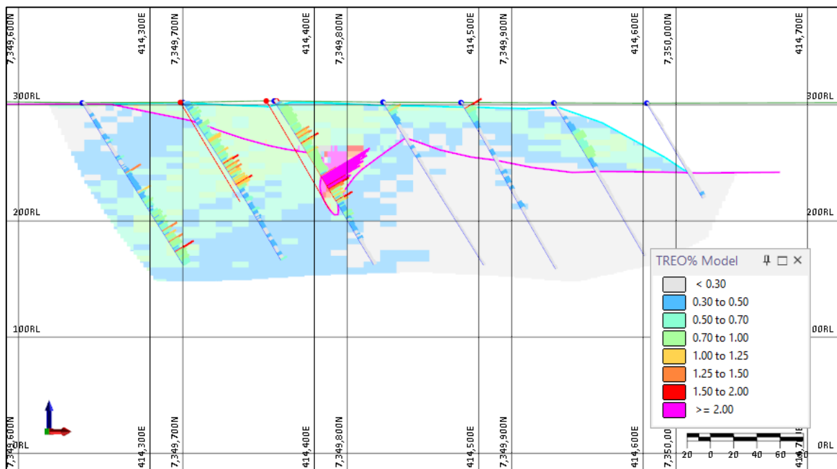
Figure 6: Section 7 showing higher grades hosted within a zone of deeper weathering (karst).
