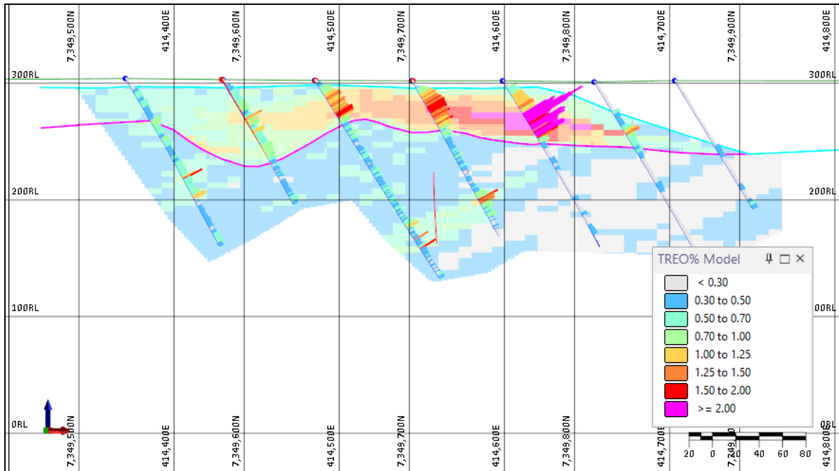
Figure 5: Section 5 showing the grade distribution within the Resource model with mineralisation near surface.
