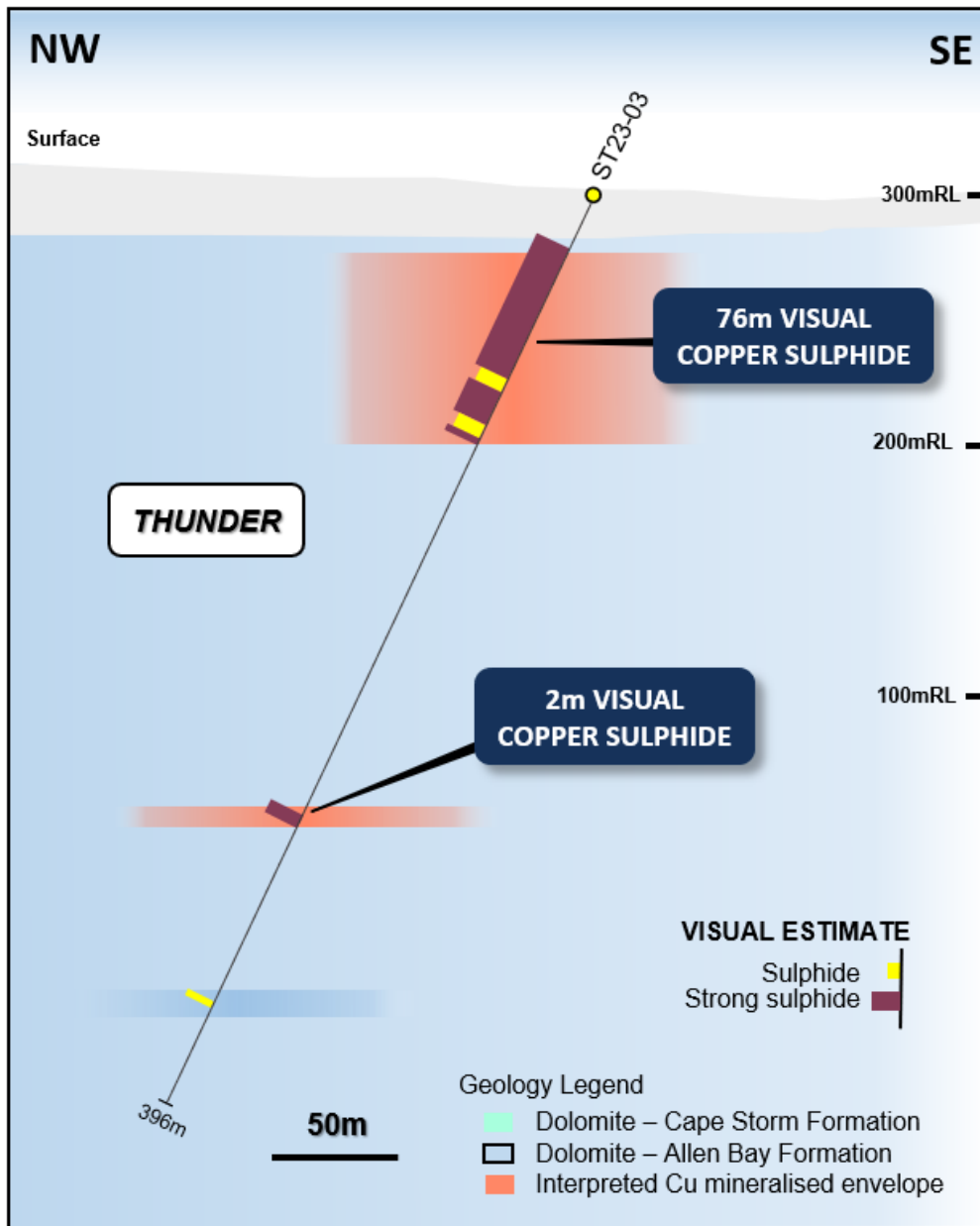
Figure 6: NW – SE geological section through drill hole ST23-03.
