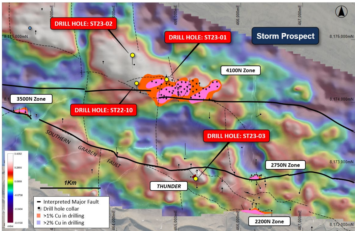
Figure 3: Total bouguer gravity image of the Storm area, fault architecture and drill hole locations
