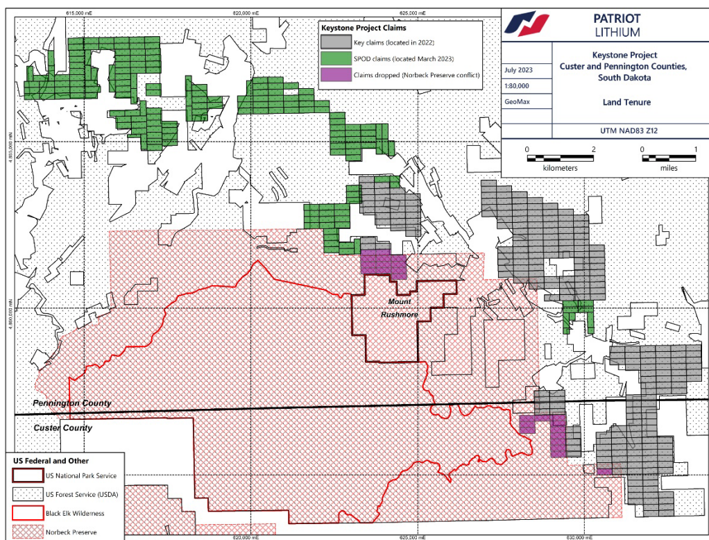
Figure 7: Keystone Tenure
