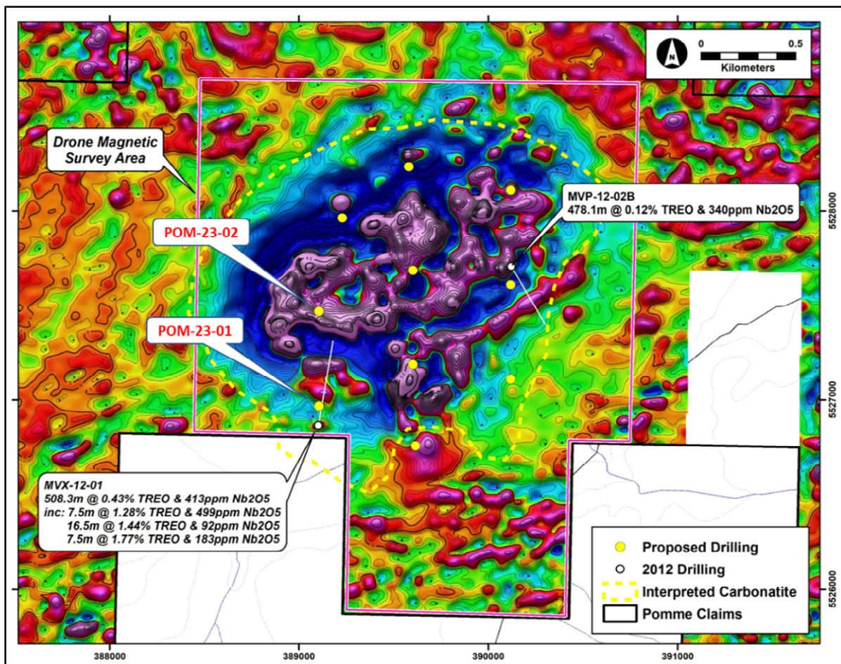
Figure 1: Diamond drilling status at the Pomme project showing historical and current diamond drill hole collar locations overlain over magnetic image (TMI 1VD) that highlights the interpreted carbonatite host rocks.
