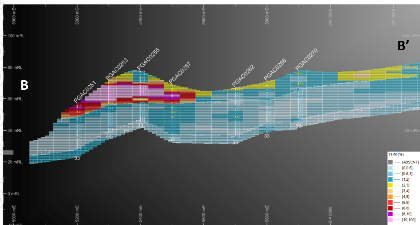
Figure 15: Cross section through western area showing drilling and block model coloured on THM grade (5x vert ex)
