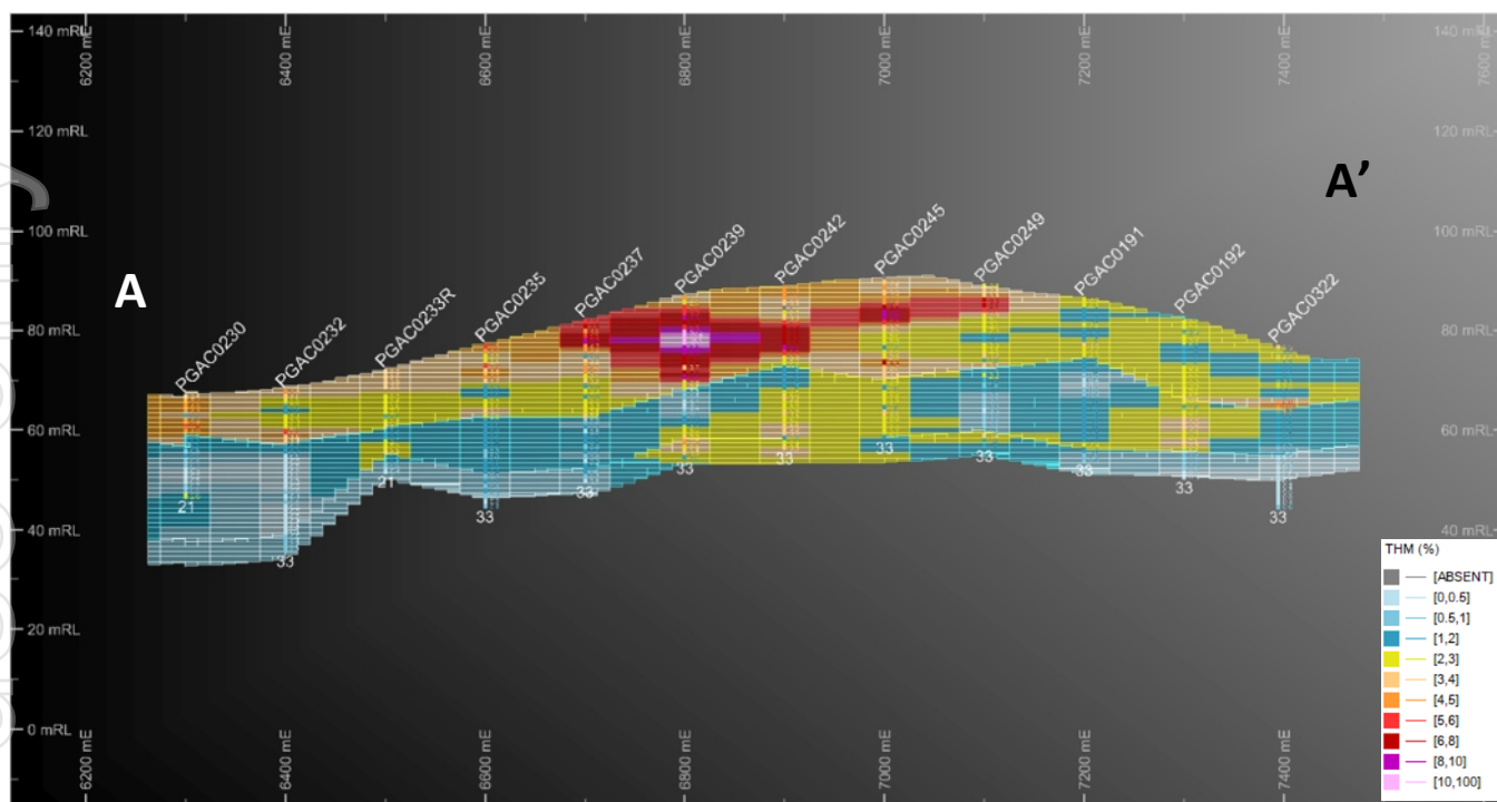
Figure 14: Cross section through eastern area showing drilling and block model coloured on THM grade (5x vert ex)
