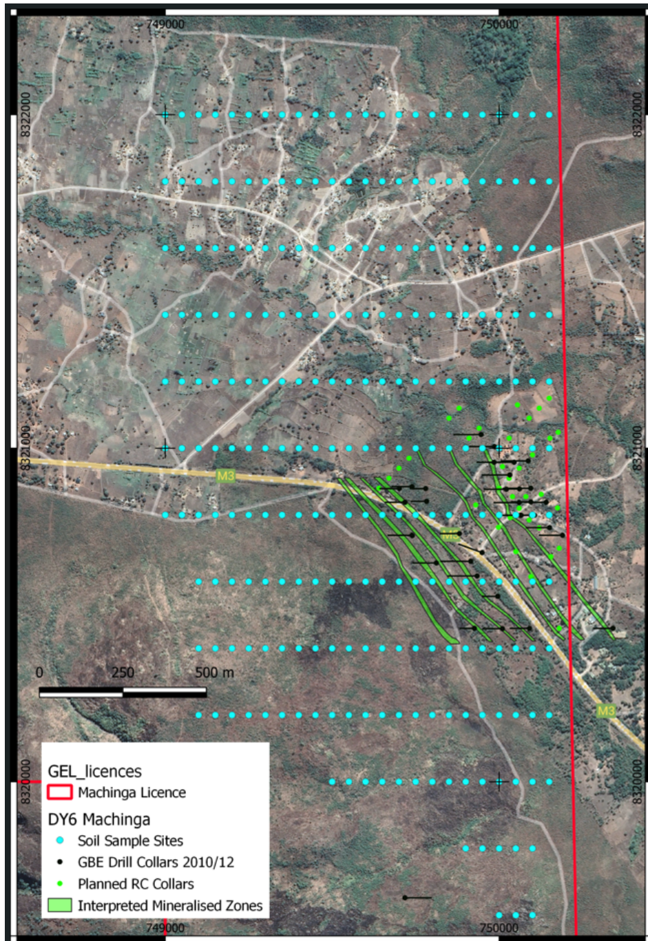
Figure 2: Soil Sample locations and Planned Collars for RC Drill Program at Machinga North.
