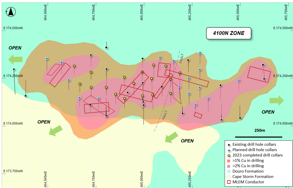
Figure 5: Plan view of the 4100N Zone showing interpreted copper mineralisation footprint (defined by drilling, MLEM and VTEM), and completed and planned drilling.
