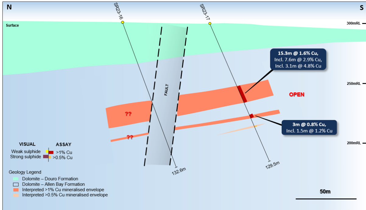
Figure 3: Geological section view at 465,140E showing the interpreted mineralisation envelopes (>0.5% & >1% Cu) and recent drill hole assays.
