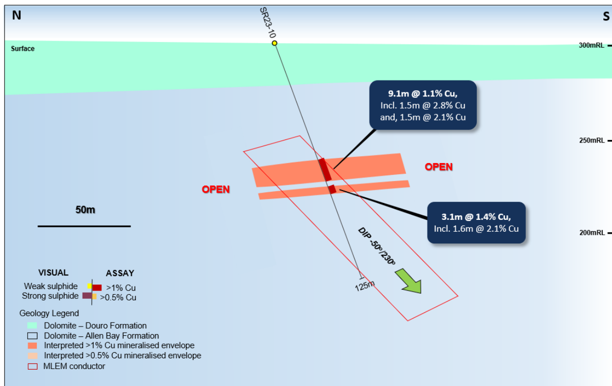
Figure 2: Geological section view at 464,64E showing the interpreted mineralisation envelopes (>0.5% & >1% Cu), MLEM conductor (off section to west of drill hole) and recent drill hole assays.
