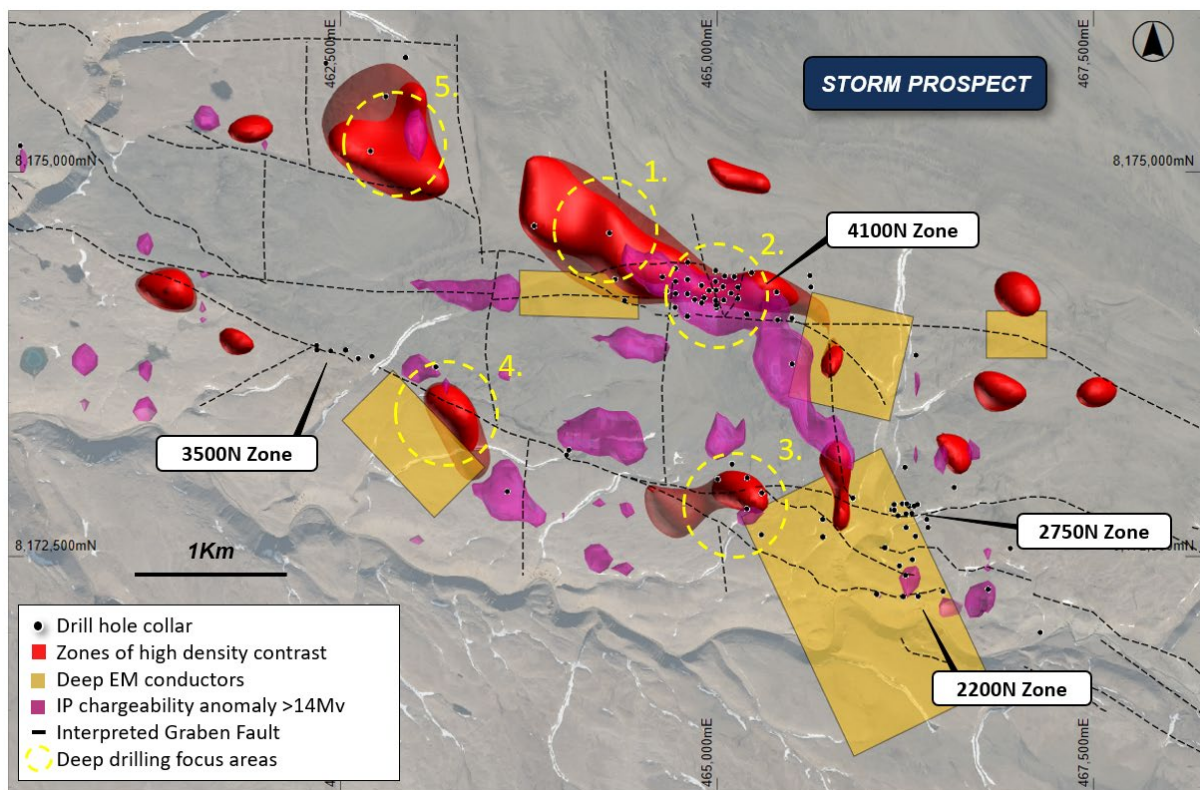
Figure 4: Geophysical interpretation map showing the focus areas (numbered) for the diamond drilling.
