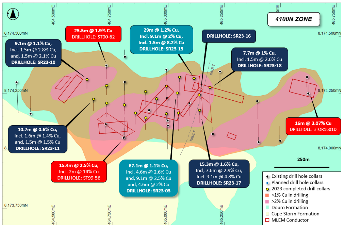
Figure 1: Plan view of the 4100N Zone showing interpreted copper mineralisation footprint (defined by drilling, MLEM and VTEM), historical and recent drilling details, overlaying regional geology.
