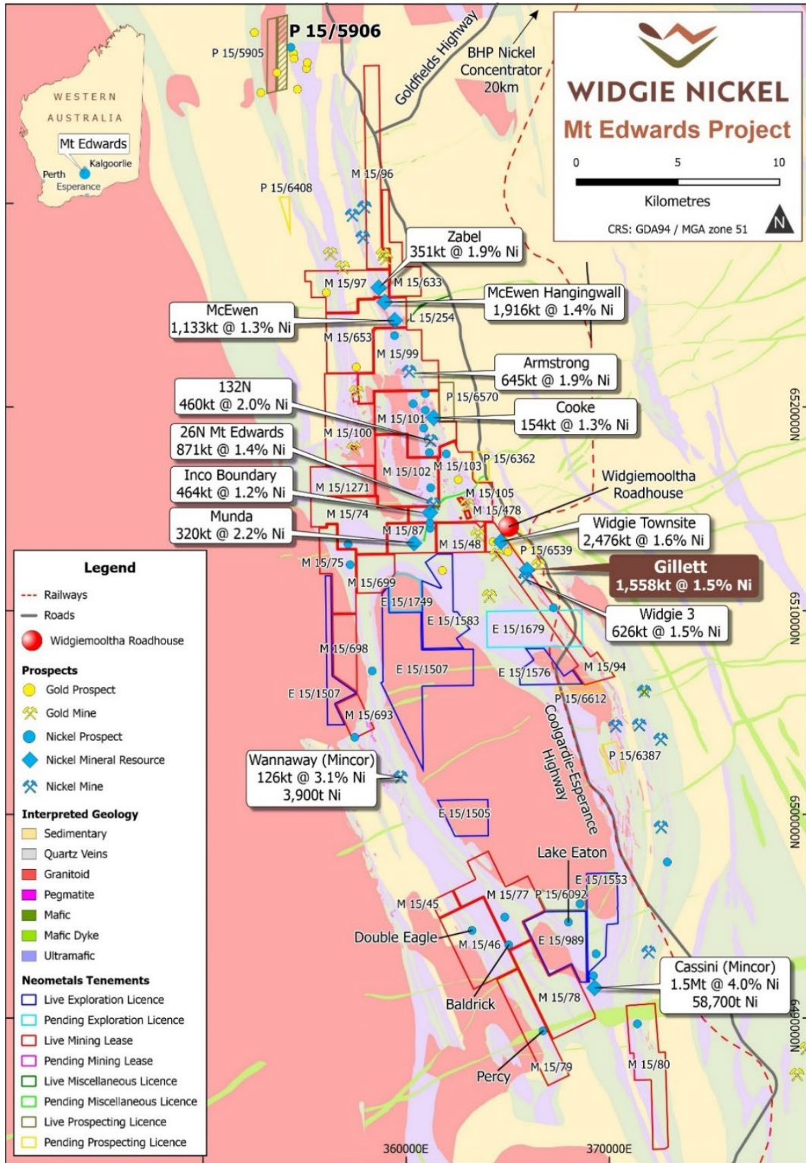
Figure 4 - Mt Edwards nickel deposits, including Munda, and surrounding nickel deposits
