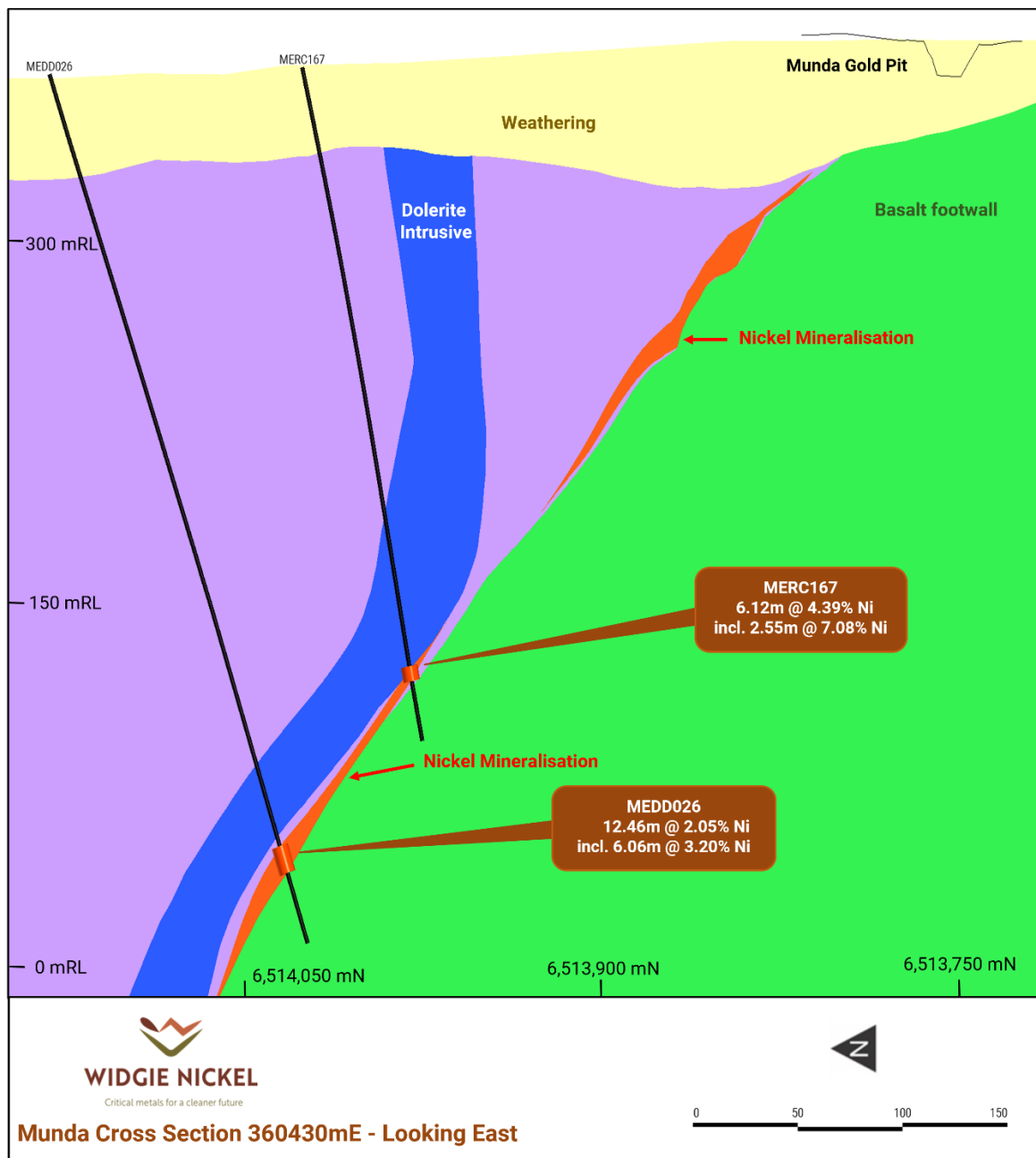
Figure 2 - Munda cross section 360430mE, drillholes MERC167 and MEDD026
