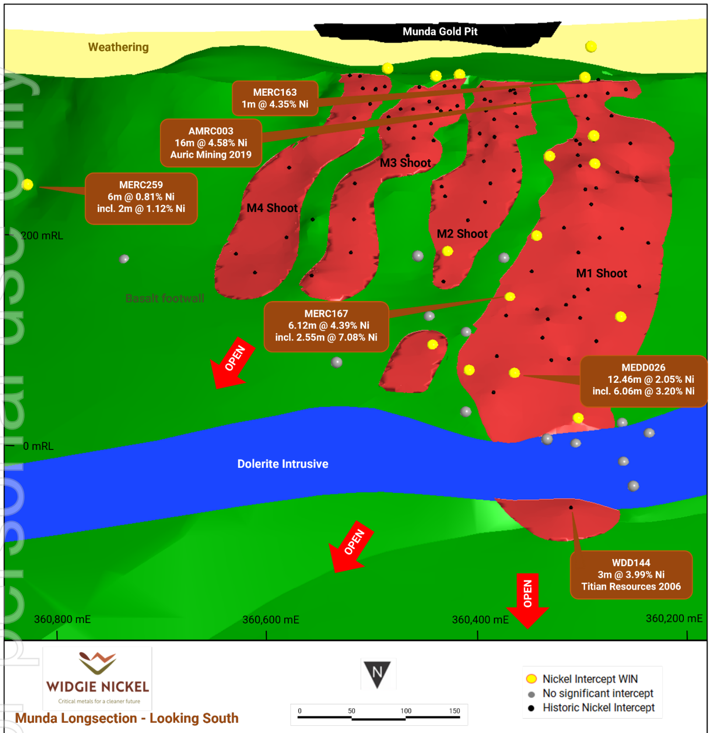
Figure 1 – Munda longsection looking South – 2023 Geology interpretation with Widgie Nickel (WIN) and historic significant intercepts
