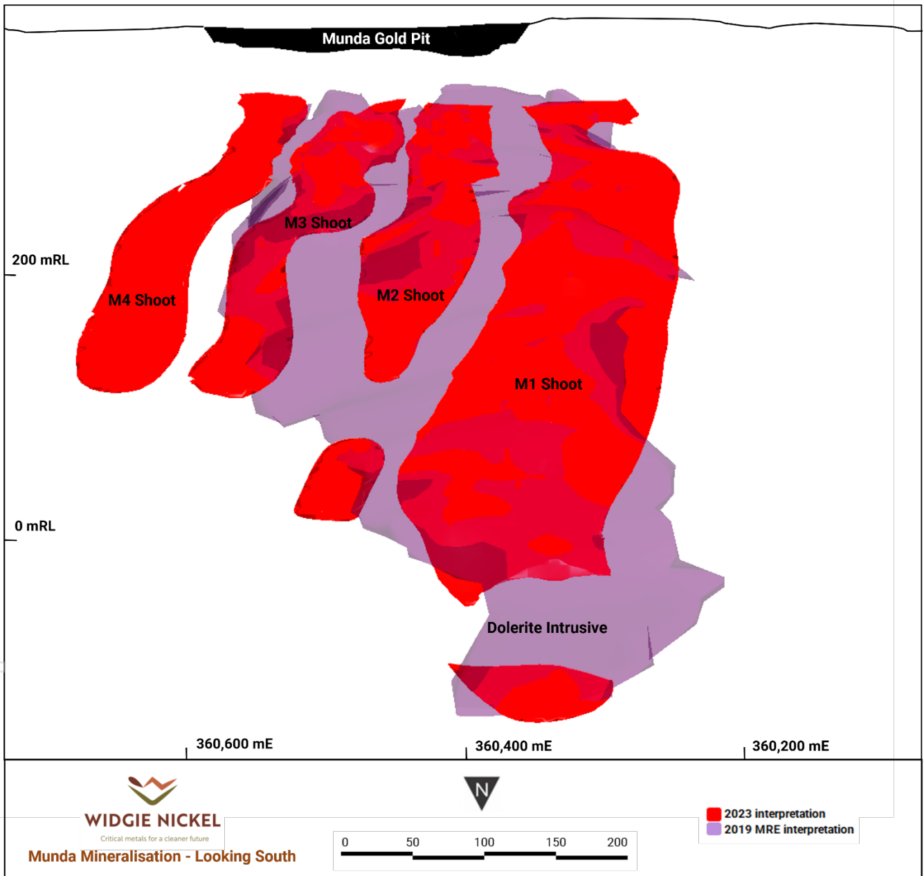
Figure 3 - Munda geological model comparison 2019 MRE (purple) 2023 interpretation (red)
