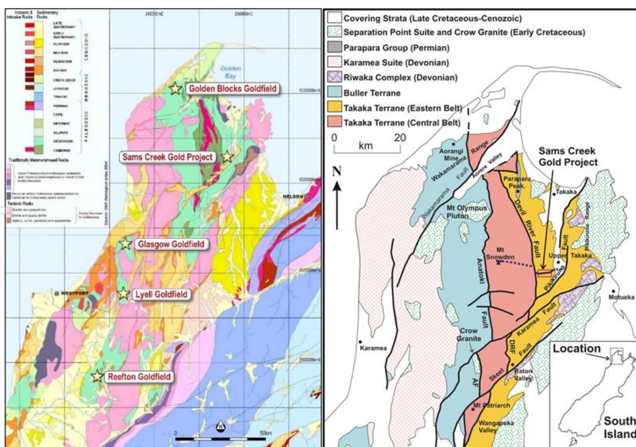
Figure 1. Top of the South Island, geology showing Palaeozoic rocks in green. Adapted from Cooper and Tulloch 1992 1 .
