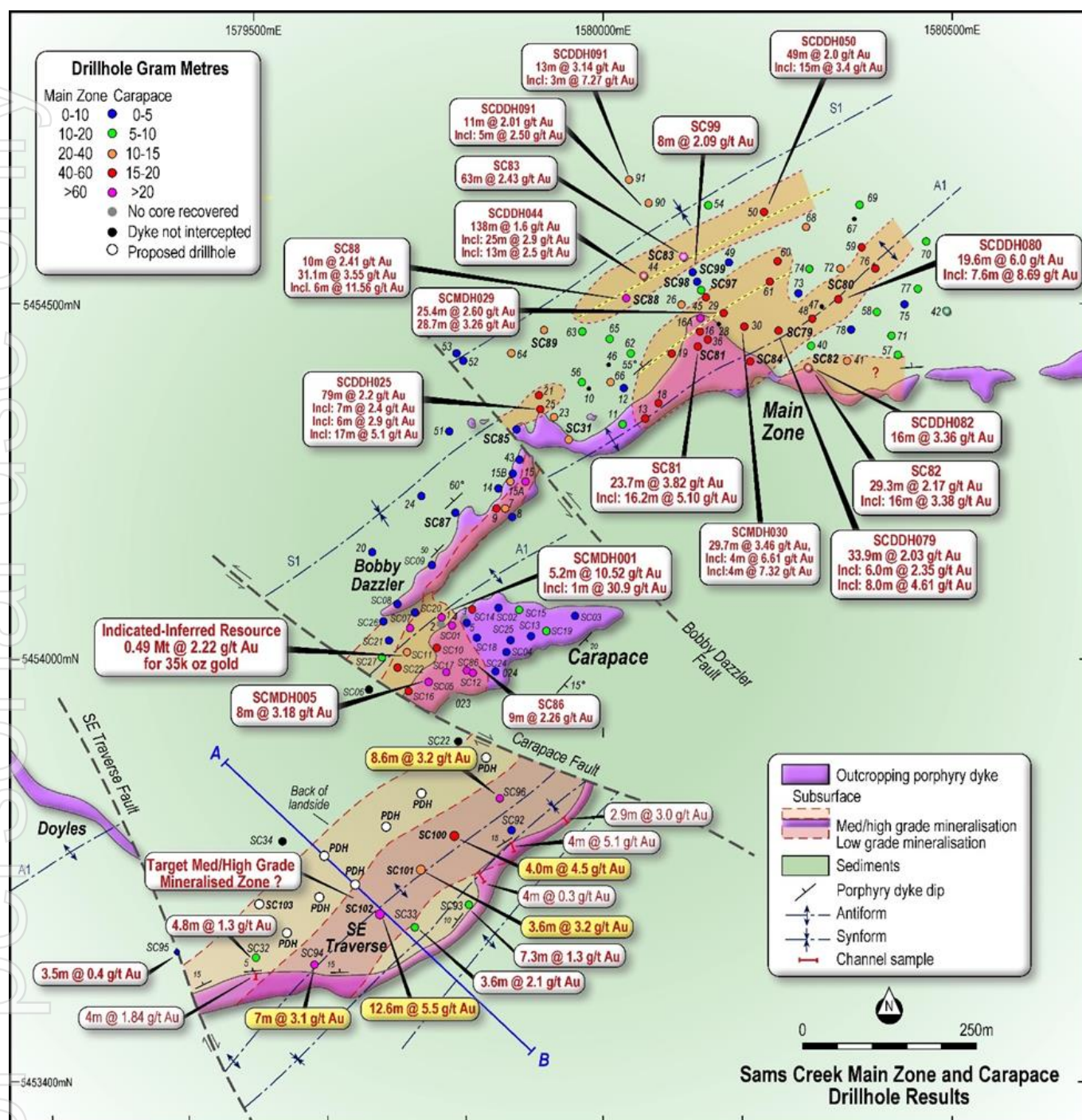
Figure 6. Plan view from SE Travers to Main Zone showing NE trending shoots.
