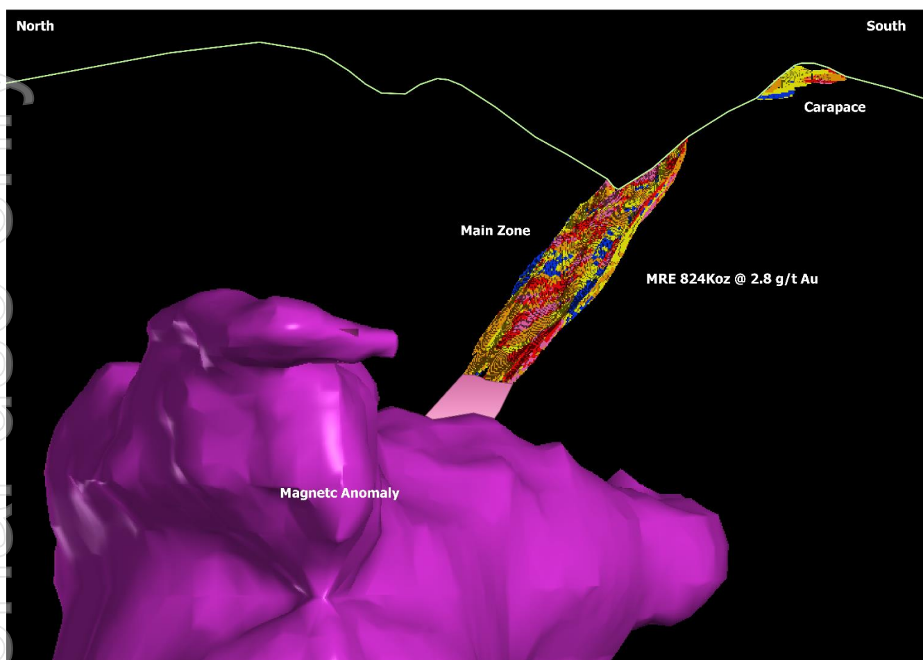
Figure 9. 3D Image of the SCD MRE and magnetic anomaly.
