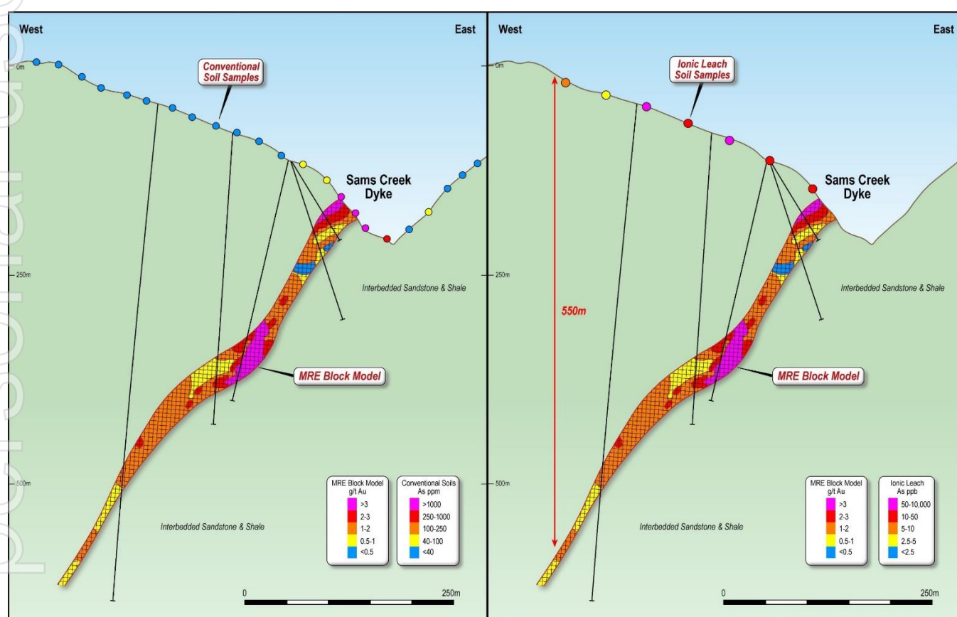
Figure 10. Cross-section showing conventional arsenic (ppm) and Ionic Leach (ppb) soils overlying the Sams Creek MRE block model.
