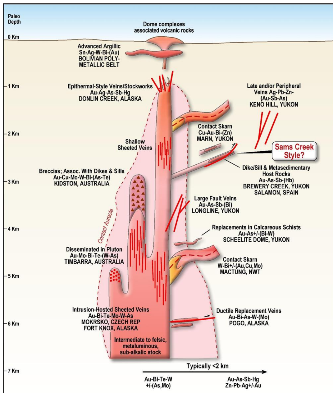
Figure 3. IRGD schematic from Lang & Baker (2001).
