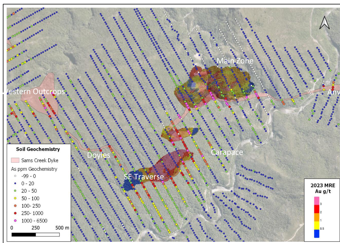
Figure 11. Conventional soil sample locations displaying arsenic ppm overlying the Sams Creek MRE block model.
