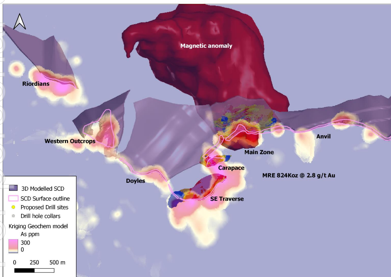
Figure 8. Arsenic soil geochemistry, SCD wireframe (grey), MRE block model and Magnetic anomaly.
