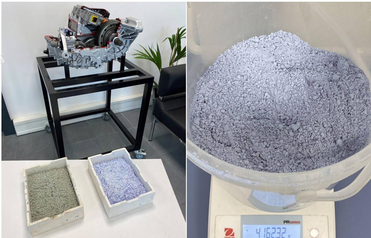
Figure 3: Left, image shows first NdPr oxide and \text{Nd}_2\text{O}_3 product laid out in Ionic Technologies showroom in front of a permanent magnet synchronous motor (PMSM), and right, >99.5% grade \text{Nd}_2\text{O}_3 product on right.
