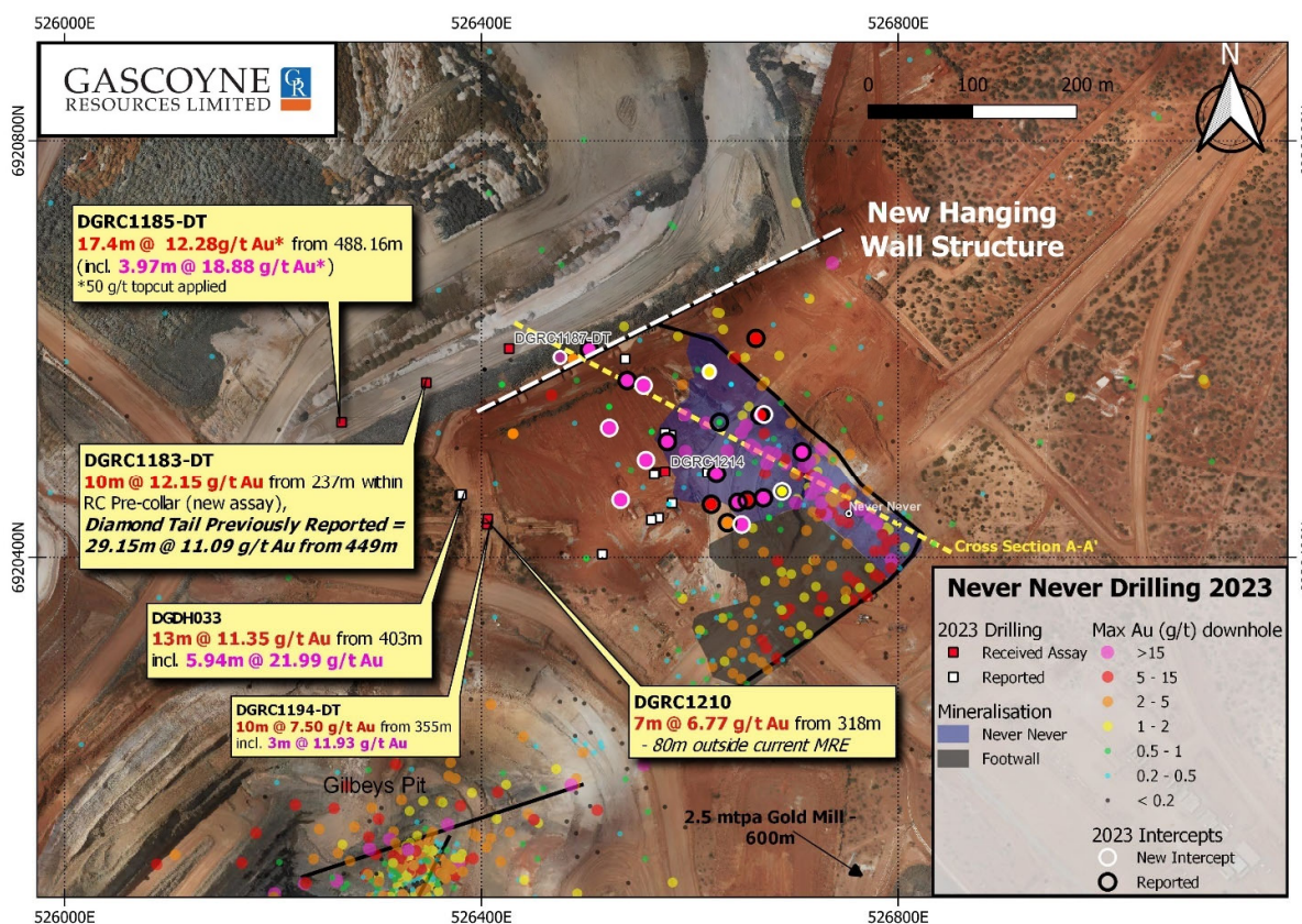
Figure 3: Plan view of the Never Never Gold Deposit (purple) with the plunge/strike in line with the yellow dashed section line. The footwall "lower grade" Gilbey's sedimentary sequence can be traced from bottom left (Gilbey's Pit) to mid right, the high-grade Never Never structural system sits at right angles to the Gilbey's stratigraphy and the new "hangingwall structure" appears to run sub-parallel to the stratigraphy but also sub-parallel to the "G-Fin" structural high-grade target (solid black line) at the north end of the Gilbey's Pit. Our geology team is currently following up both the "G-Fin" and "hangingwall structure" with a Diamond drill-rig.
