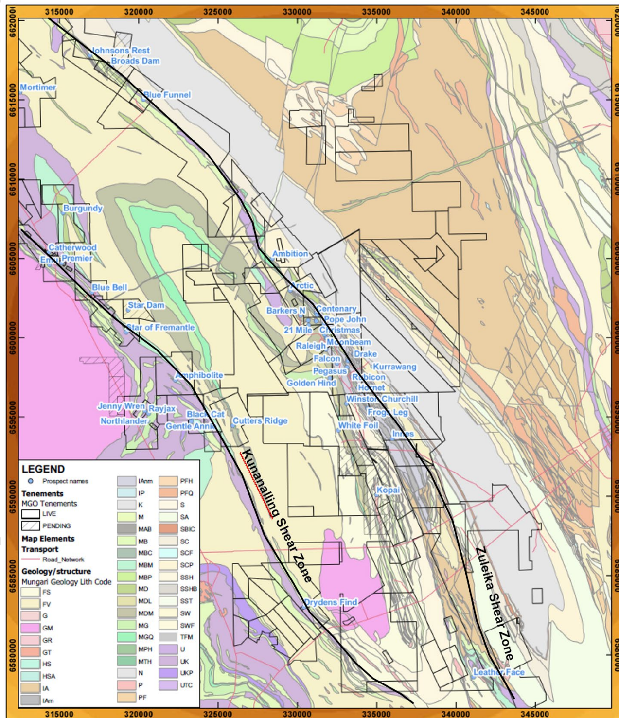
Figure 4. The Kundana project area sub-surface Geology
