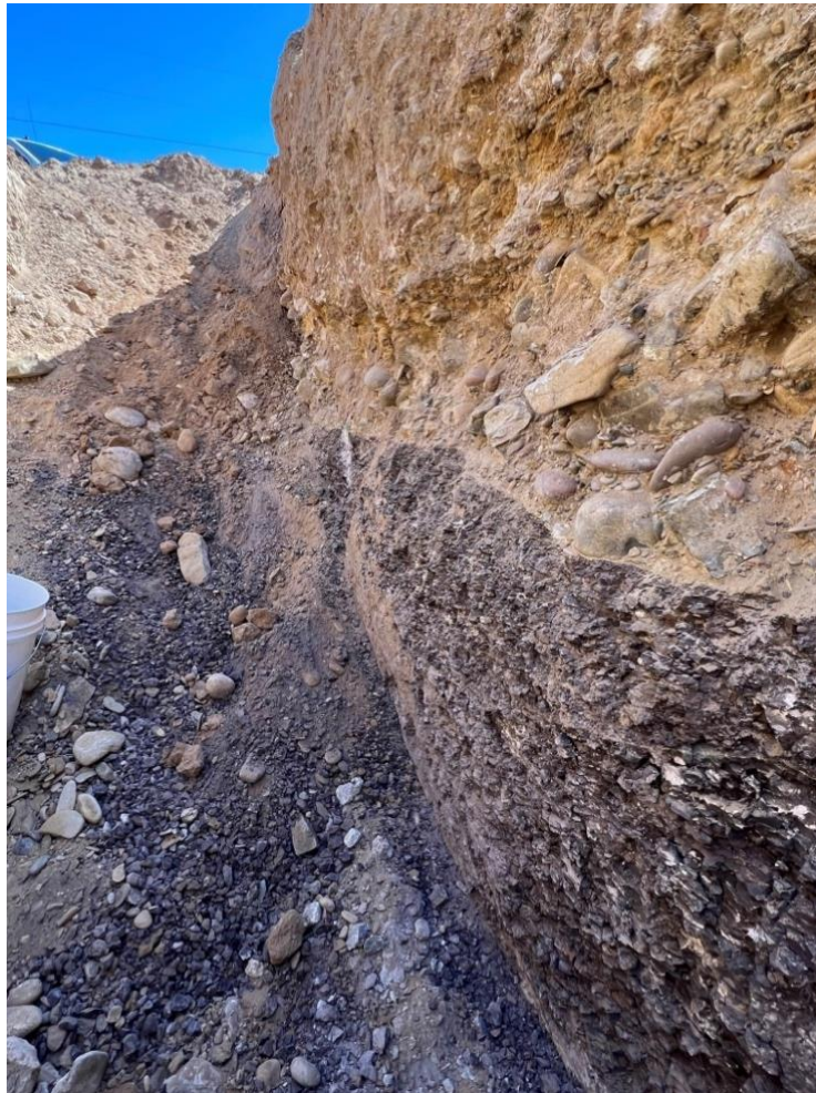
Figure 3: One of the Green River site trenches showing soils for foundations with shallow bedrock & dense gravels.
