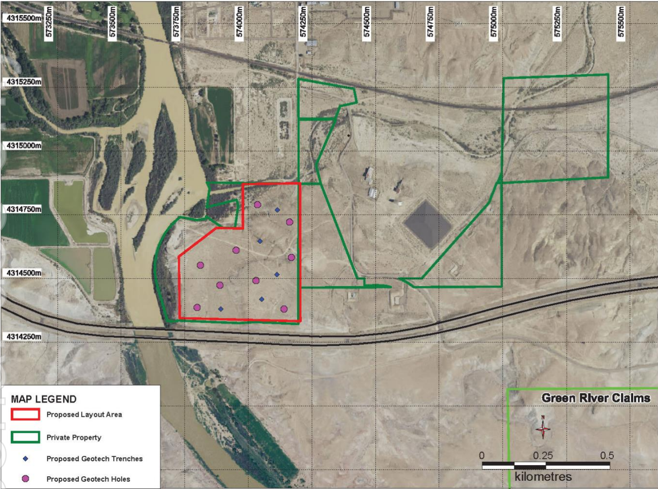
Figure 2: Plan showing the locations of the proposed boreholes and test pits.
