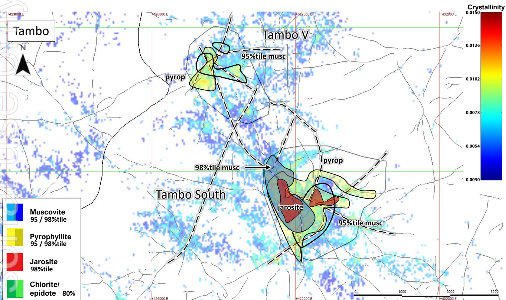
Figure 10: Image showing muscovite crystallinity as deduced from ASTER data and vectors for the linear zones of iron-oxide – kaolinite – phyllic alteration (wavelength – 100m) at Tambo South and Tambo V. The degree of muscovite crystallinity is indicated by color, with highly crystalline mica (high temperature) designated as red and poorly crystalline mica (lower temperature) shown as blue. Three major zones of higher crystallinity (higher temperature) are interpreted. The Tambo South muscovite zone is of high crystallinity, which is consistent with the interpretation of a proximal porphyry centre; the crystallinity of Tambo V centre is of a lower magnitude, which may suggest a more distal setting. The dashed lines indicate interpreted structures (faults / fracture zones) that are inferred to control hydrothermal alteration and metals distribution (cf. previous figure).
