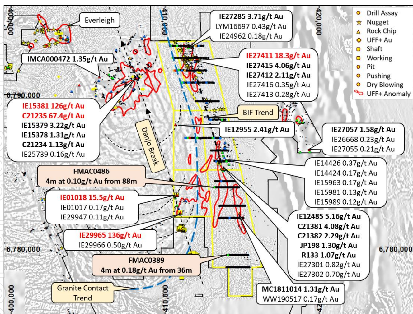
Figure 1 Gold rock chip assays across the Guyer Well target area and the Guyer South AC results.
