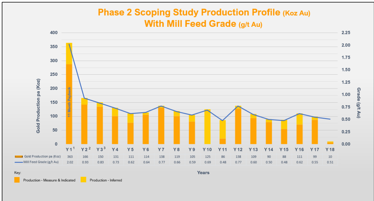
Figure 3. Annual production profile
