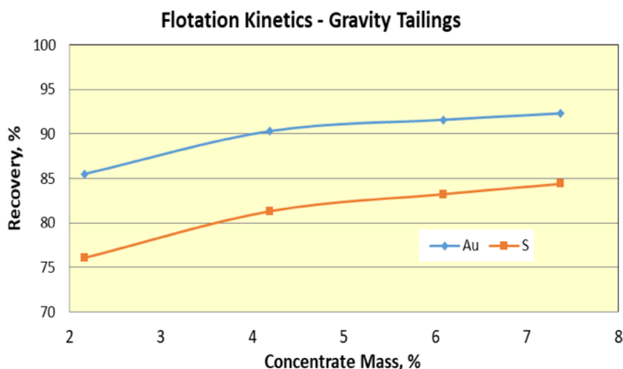
Figure 21. Flotation kinetics
