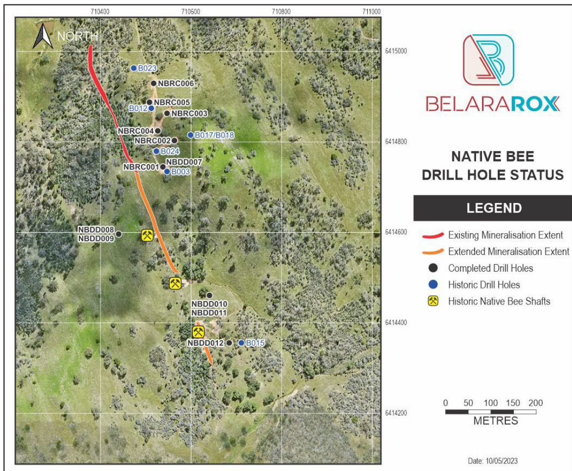
Figure 1. Phase 2 completed drill holes NBDD007-NBDD012 over aerial imagery. Note the Native Bee historical shaft locations.
