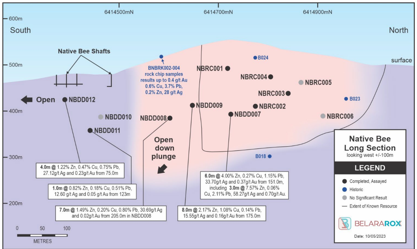
Figure 2. Long section at Native Bee showing drill intersections from Phase 2 drilling. Note that mineralisation remains open down plunge.
