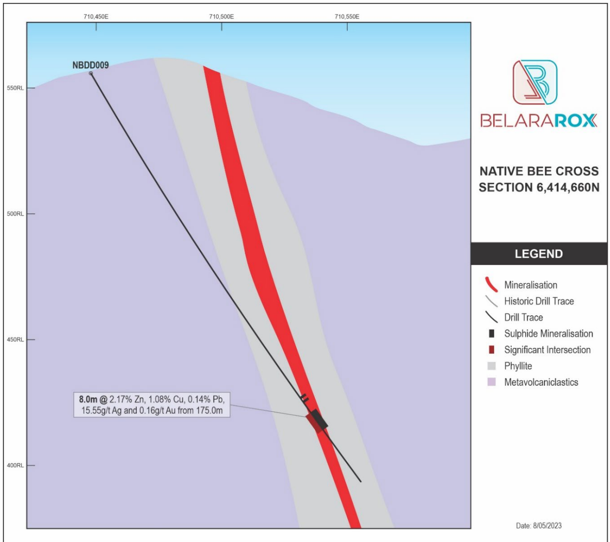
Figure 4. Cross section looking north at Native Bee showing drill intersection from NBDD009.
