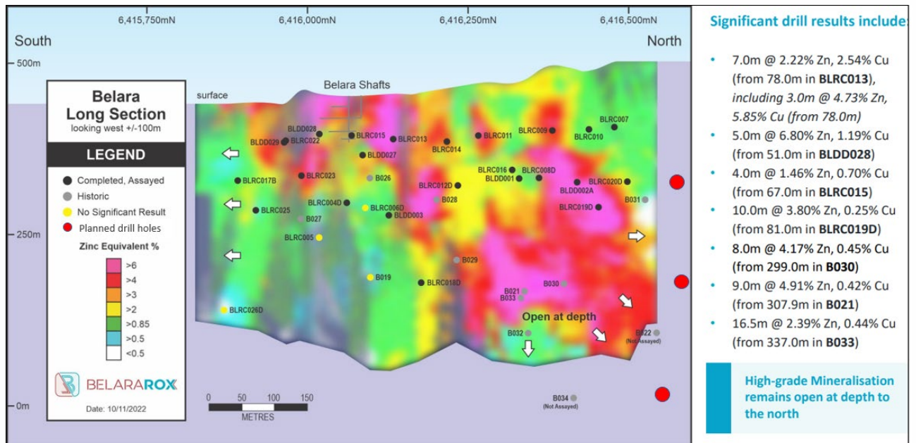
Figure 7. Long section at Belara showing existing drill intersections and planned mineralisation intersections for Phase 2 drilling
