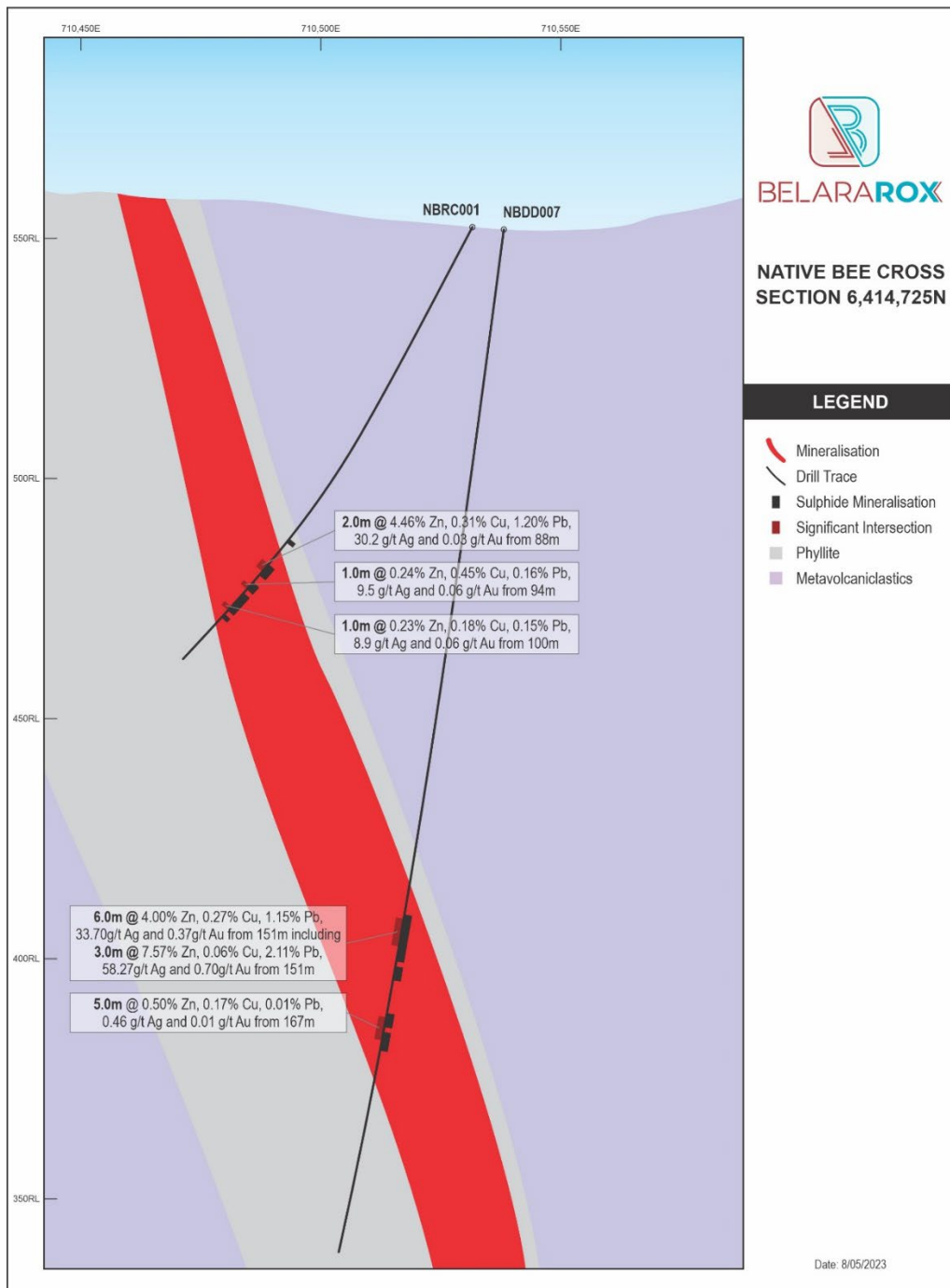
Figure 3. Cross section looking north at Native Bee showing drill intersections from NBDD007. Note that mineralisation remains open down dip and appears to be increasing in width and grade.
