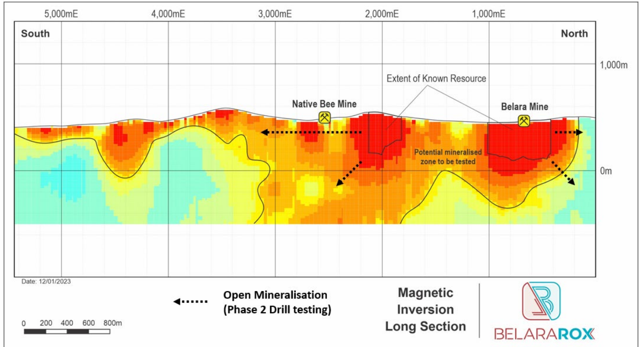
Figure 6. Long section from the Belara historic mine through the Native Bee historic mine showing the 3D magnetic inversion data and open mineralisation.
