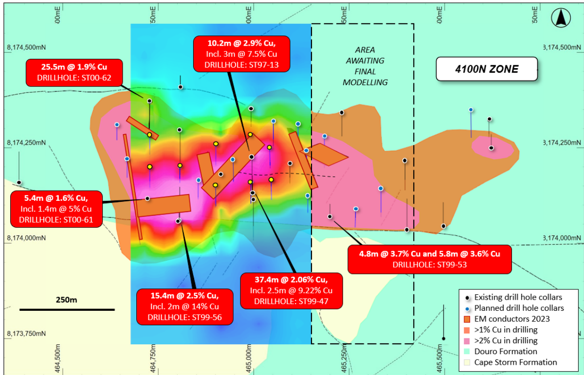
Figure 9: Plan view of the 4100N Zone indicating the location of the preliminary 2023 MLEM conductors (red) modelled to date, overlaying MLEM image (CH18Z, hotter colours are higher conductivity, cooler colours are lower conductivity - eastern extent of data still being processed) and footprint of the mineralisation defined by drilling.
