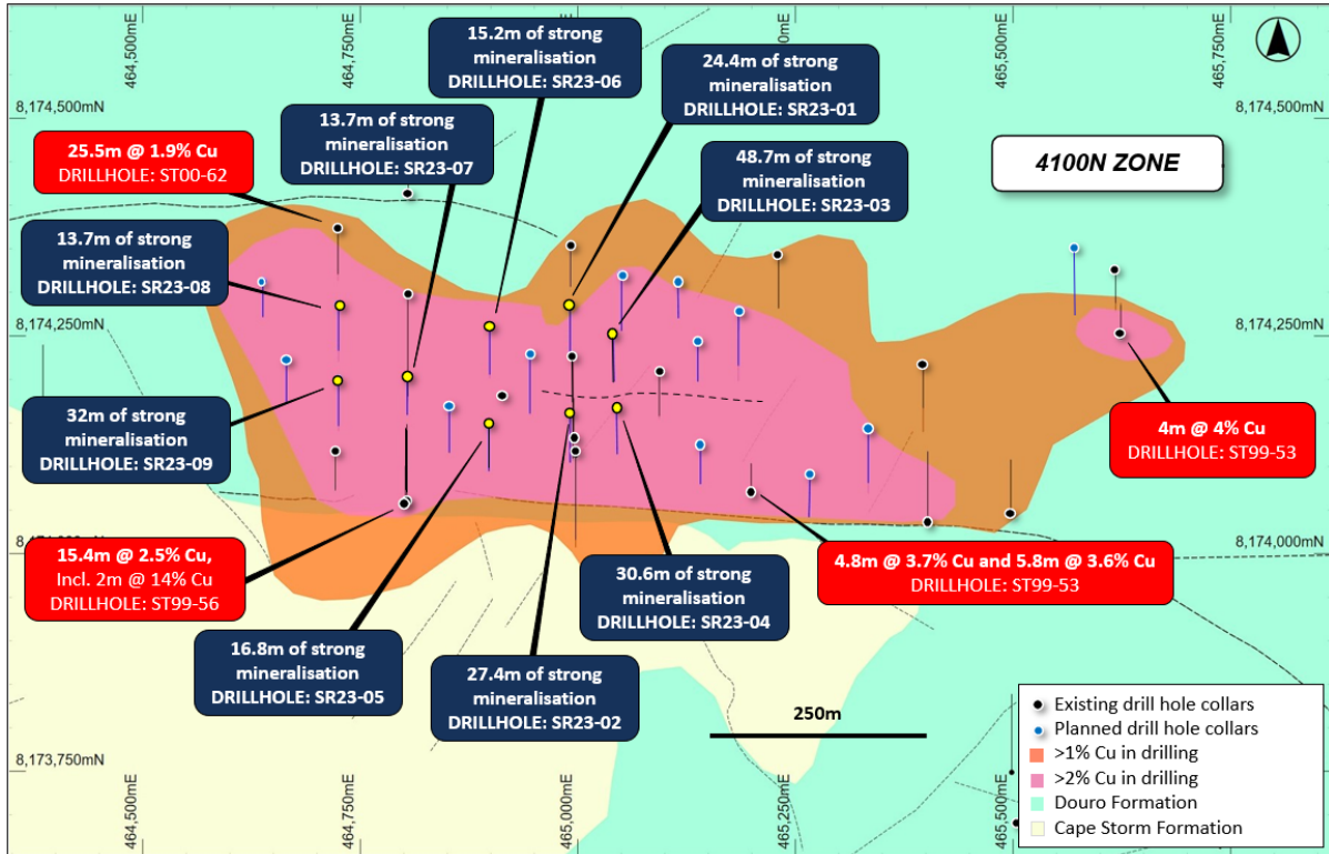
Figure 2: Plan view of the 4100N Zone showing interpreted copper mineralisation footprint (defined by drilling), historical and recent drilling, overlaying regional geology.
