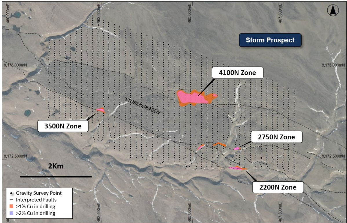
Figure 10: Plan view of the Storm Prospect area showing the completed ground gravity survey stations.
