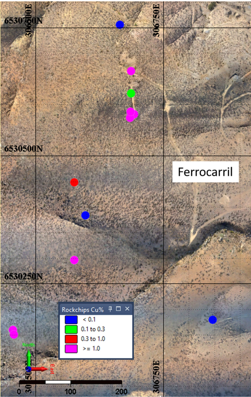
Figure 4 Ferrocarril high-grade copper veins
