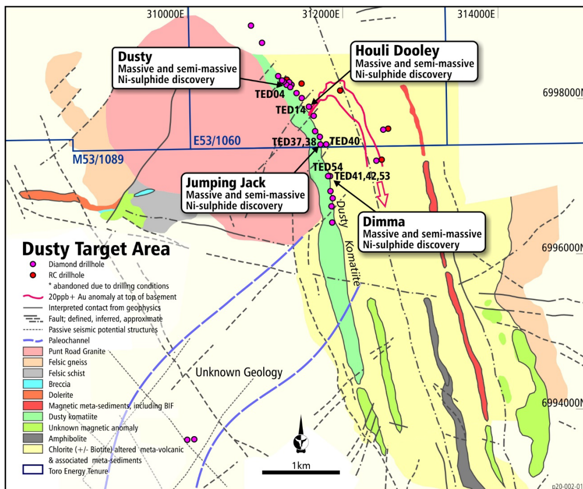
Figure 1: Location of the Dimma Ni-sulphide Discovery relative to the three other nickel sulphide discoveries within the Dusty Target Area. Note the extensive strike length of the Dusty Komatiite, at least 7.5km long.
