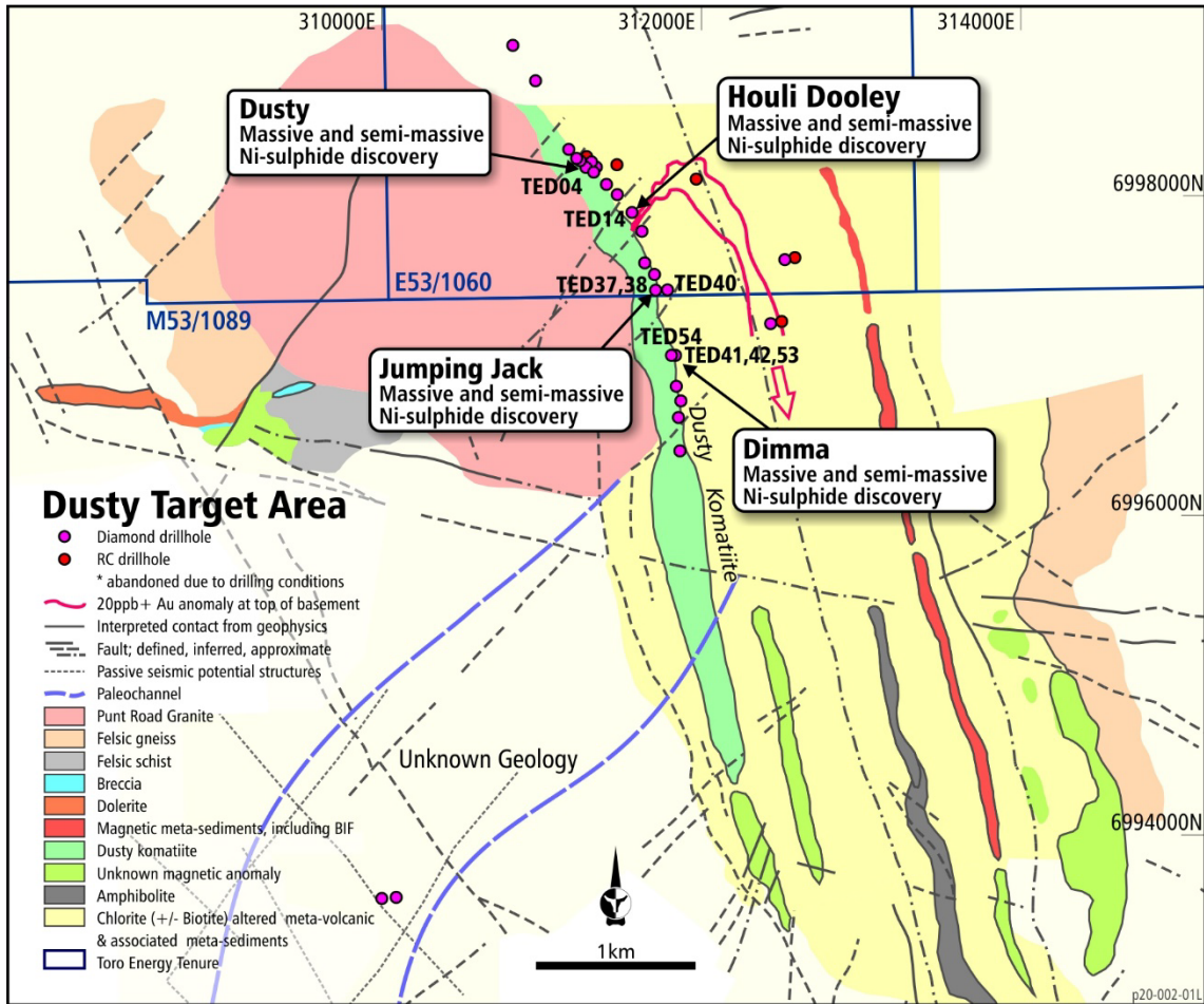
Figure 1: Location of the Dimma Ni-sulphide Discovery relative to the three other nickel sulphide discoveries within the Dusty Target Area. Note the extensive strike length of the Dusty Komatiite, at least 7.5km long.
