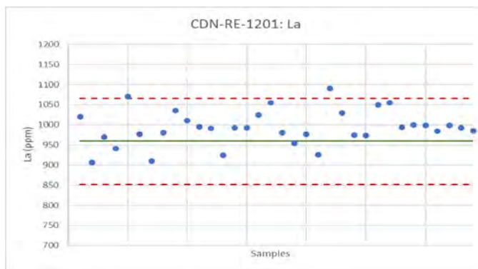
Figure 36 – Graphs of internal CRM tolerances for Ce and La: CDN-RE-1201
