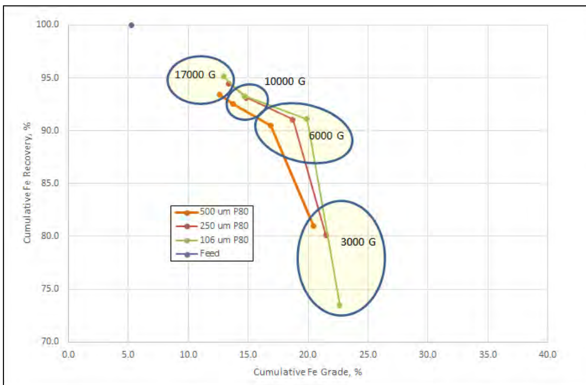
Figure 49 - Progressive Primary WHIMS Fe Grade-Recovery Plots at Three Grind Sizes
