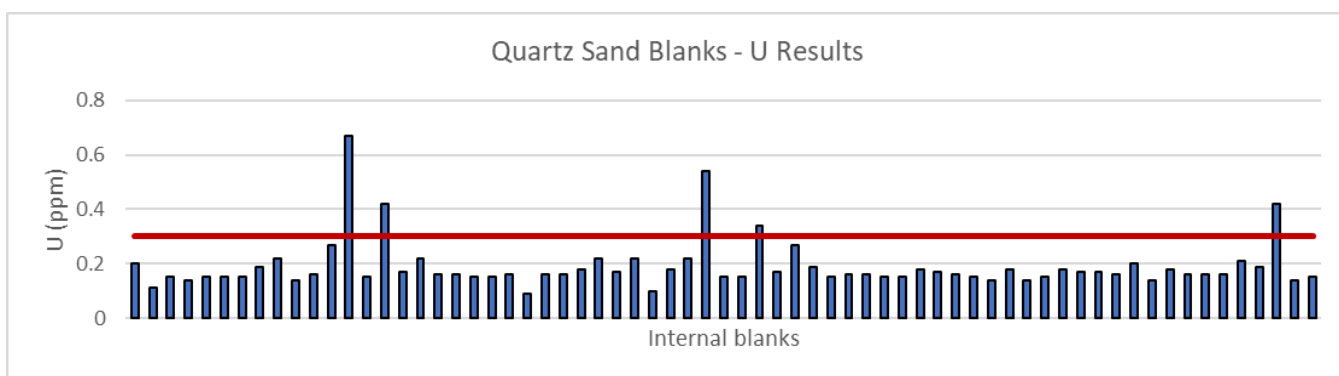
Figure 24 – Chart of internal OREAS 22-h blank for U
