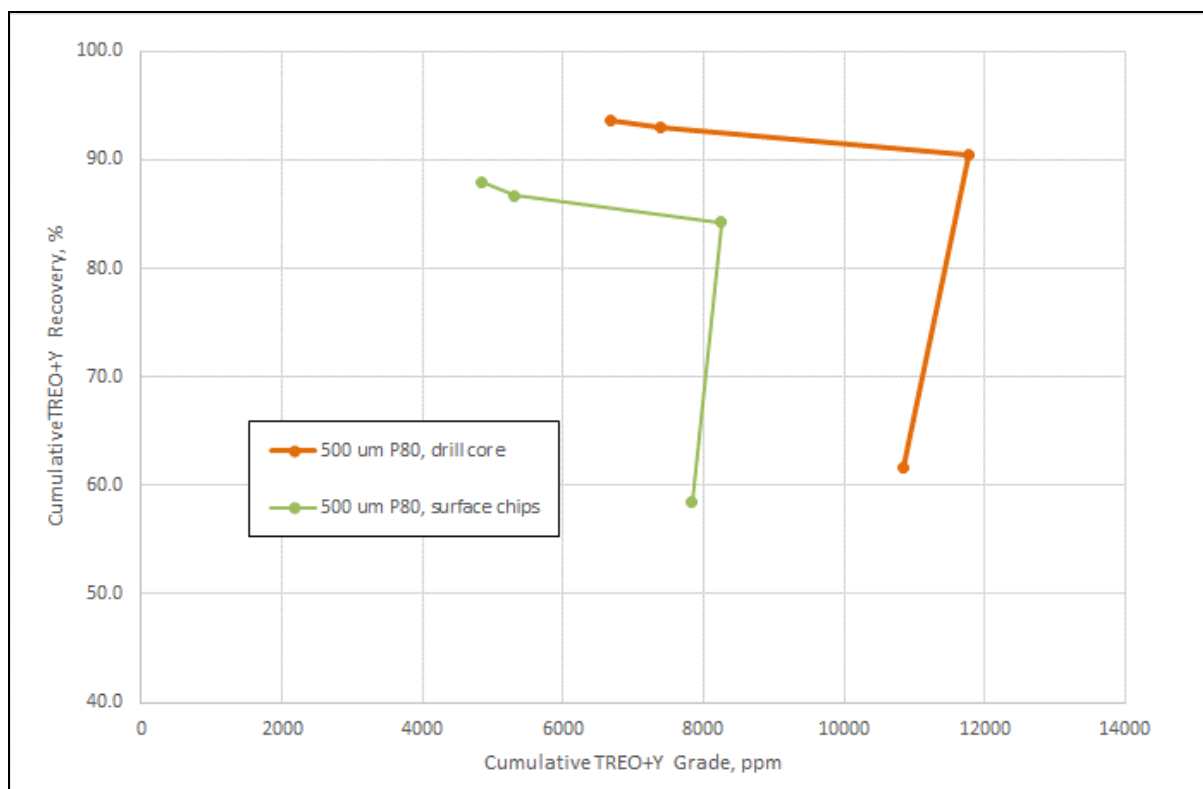
Figure 48 - Grade-Recovery Plot for Surface Chip and Drill Core Results, 500 microns P 80
