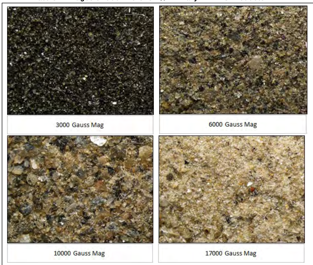
Plate 3 - Images of 500 microns P 80 Primary WHIMS Products
