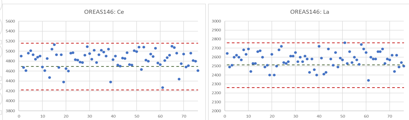
Figure 43 – Graphs of laboratory CRM tolerances for Ce and La: OREAS146
