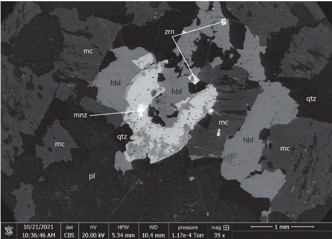
Plate 2 - Scanning electron microscope images of petrographic textures
