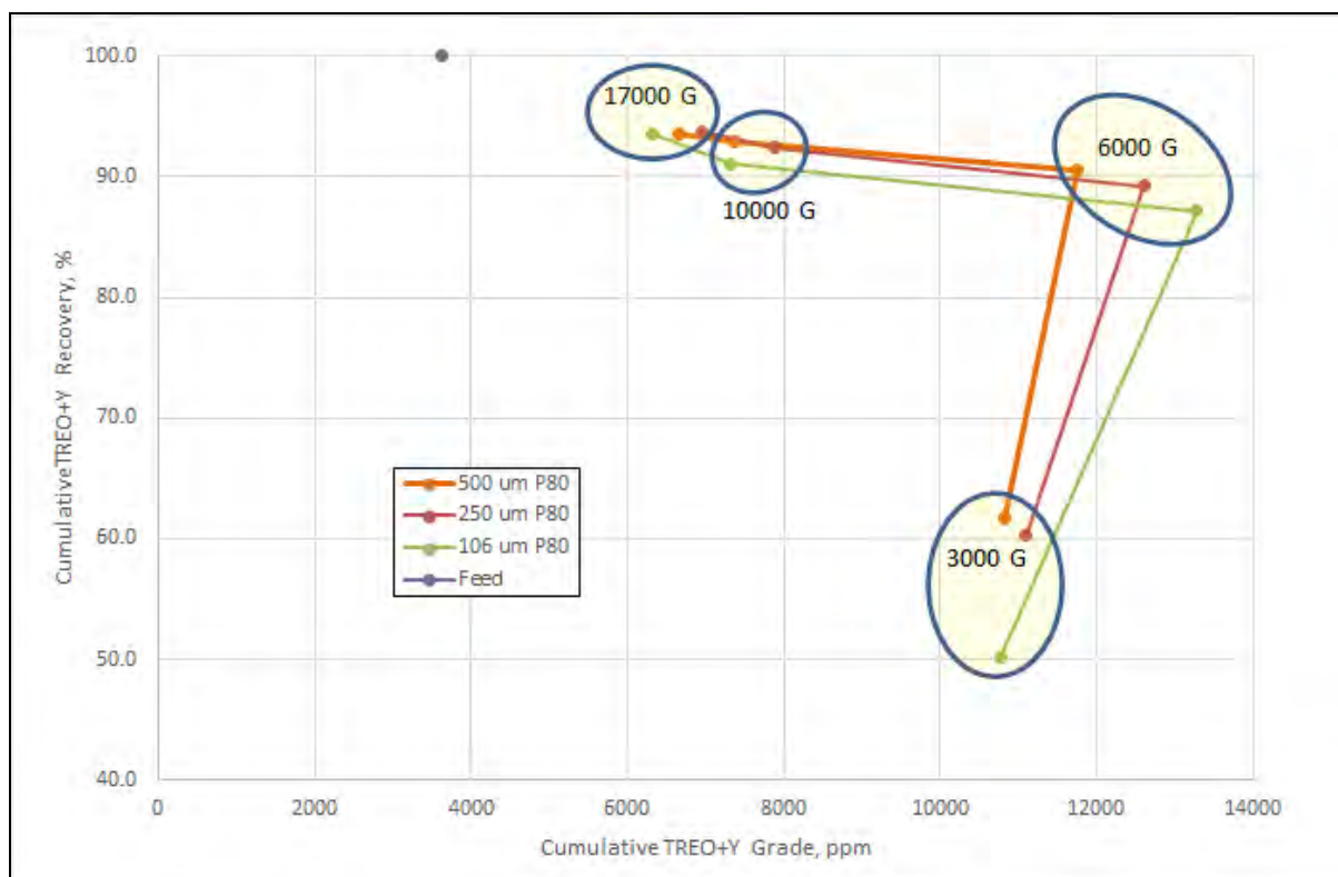
Figure 47 - Progressive Primary WHIMS TREO+Y Grade-Recovery Plots at Three Grind Sizes
