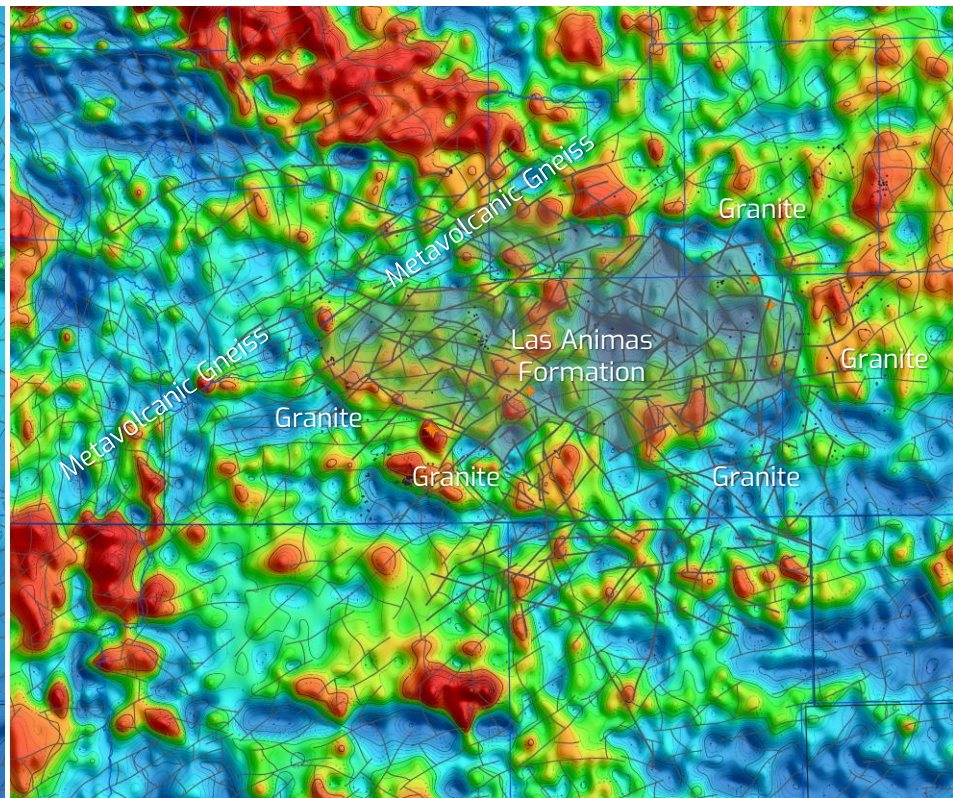
Radiogenic/Basement Composition
