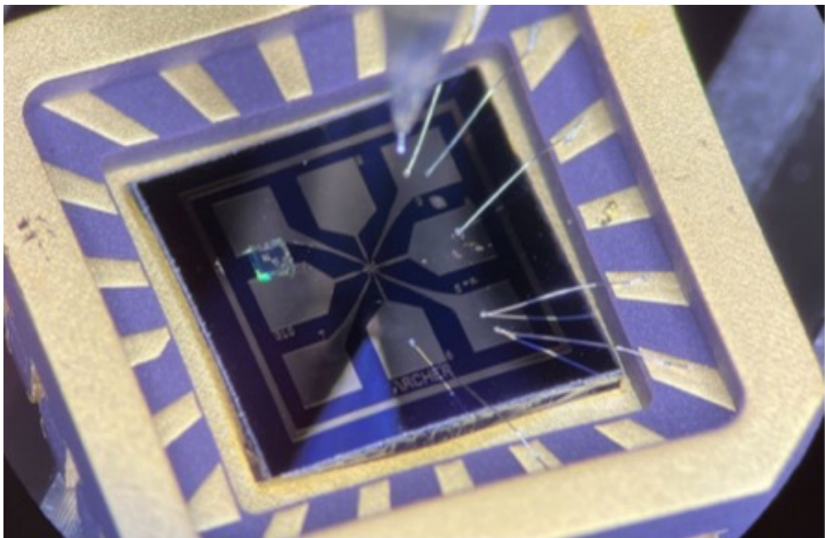
Image 2. An Archer 4 x 4 mm single-chip quantum electronic device after installing and bonding into a commercial chip carrier. This completed device is compatible with measurement setups for electronic characterisation at cryogenic temperatures as well as ambient conditions at room temperature using Archer's in-house lab capabilities as well as external facilities.
