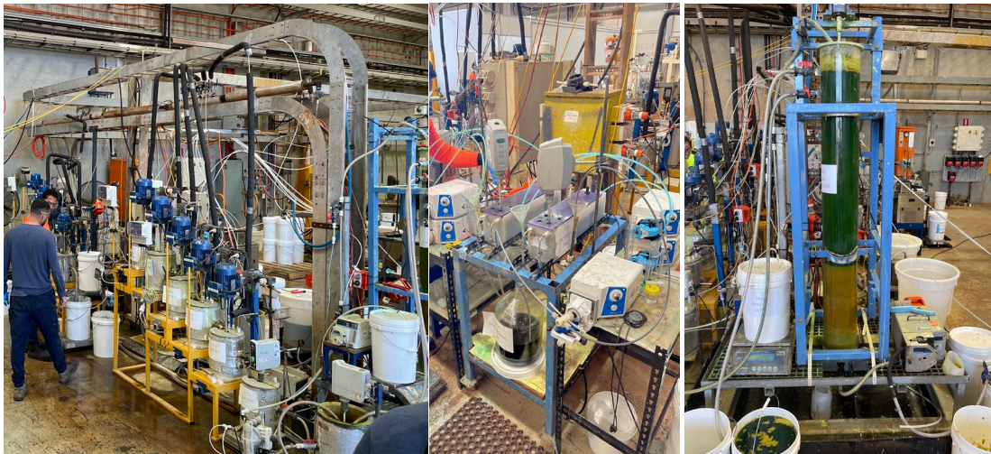
Figure 4: Primary Neutralisation, Copper Solvent Extraction and Secondary Neutralisation
