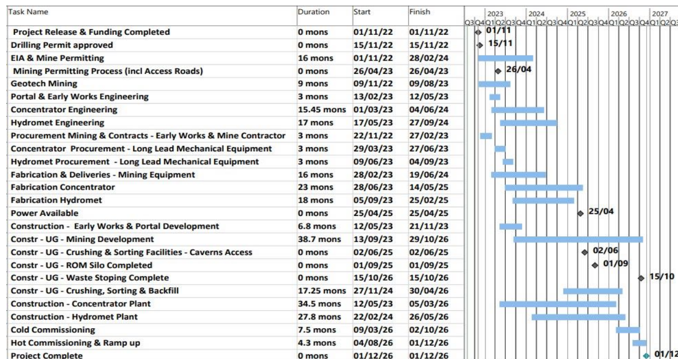
Figure 8.1.1: Project Schedule
