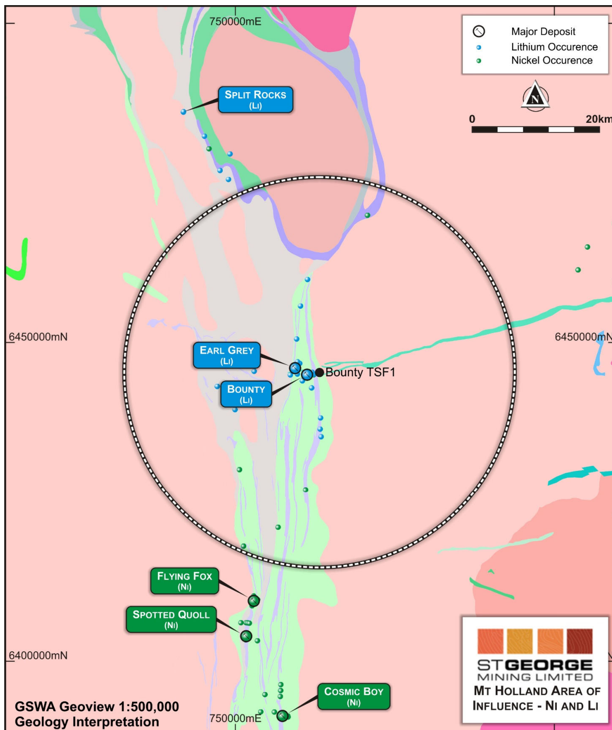
Figure 1: Interpreted geological map showing the 30km radius Area of Influence and significant known lithium and nickel occurrences and deposits along the greenstone belt
